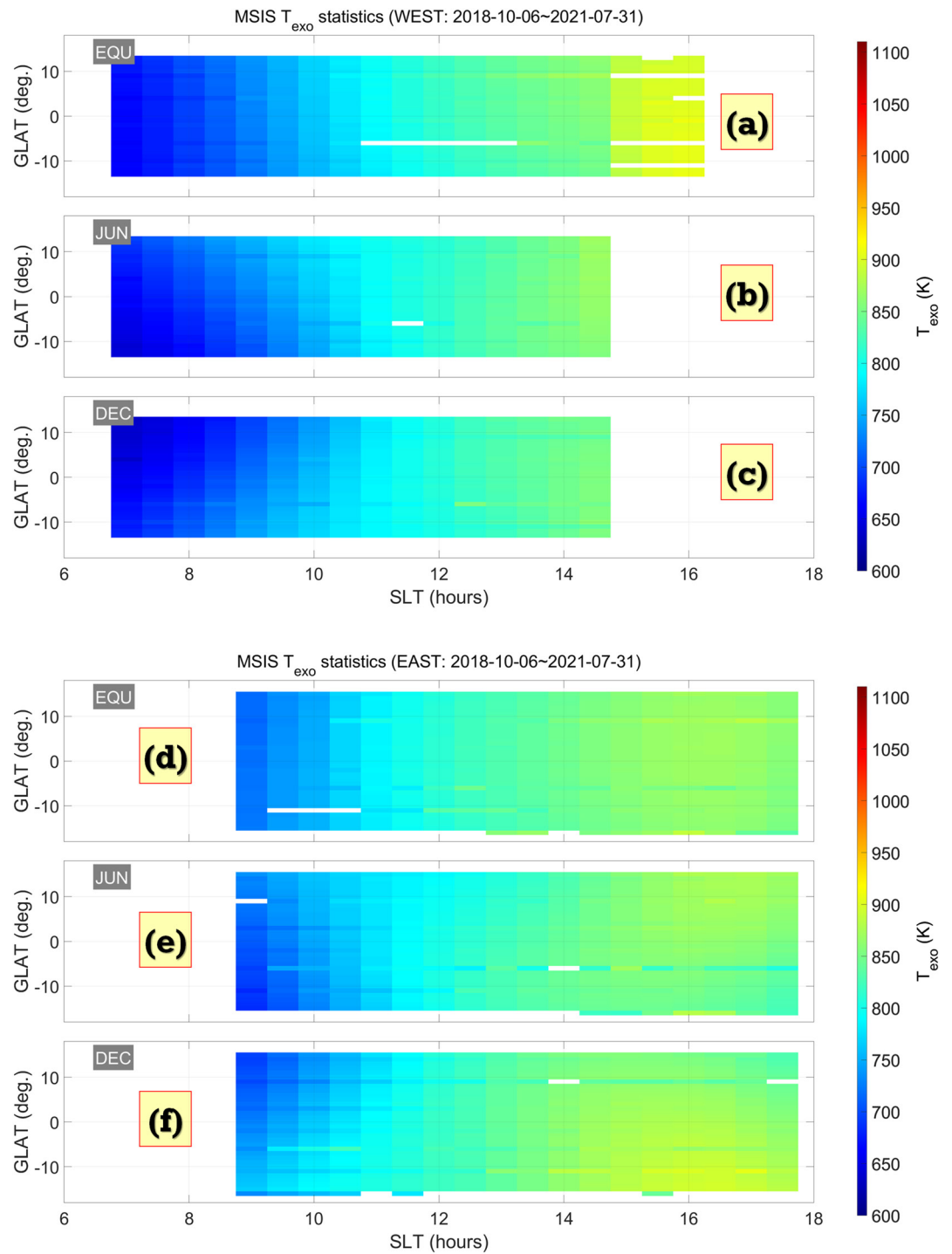
Figure 7. Similar to Figure 1, but presenting MSIS2.0 T_{\text{exo}} instead of GOLD T_{\text{exo}} .
