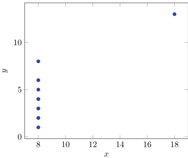
Fig. 2. Data set 2: correlation coefficient = 0.812, p -value of HSIC based statistical test = 0.9.
