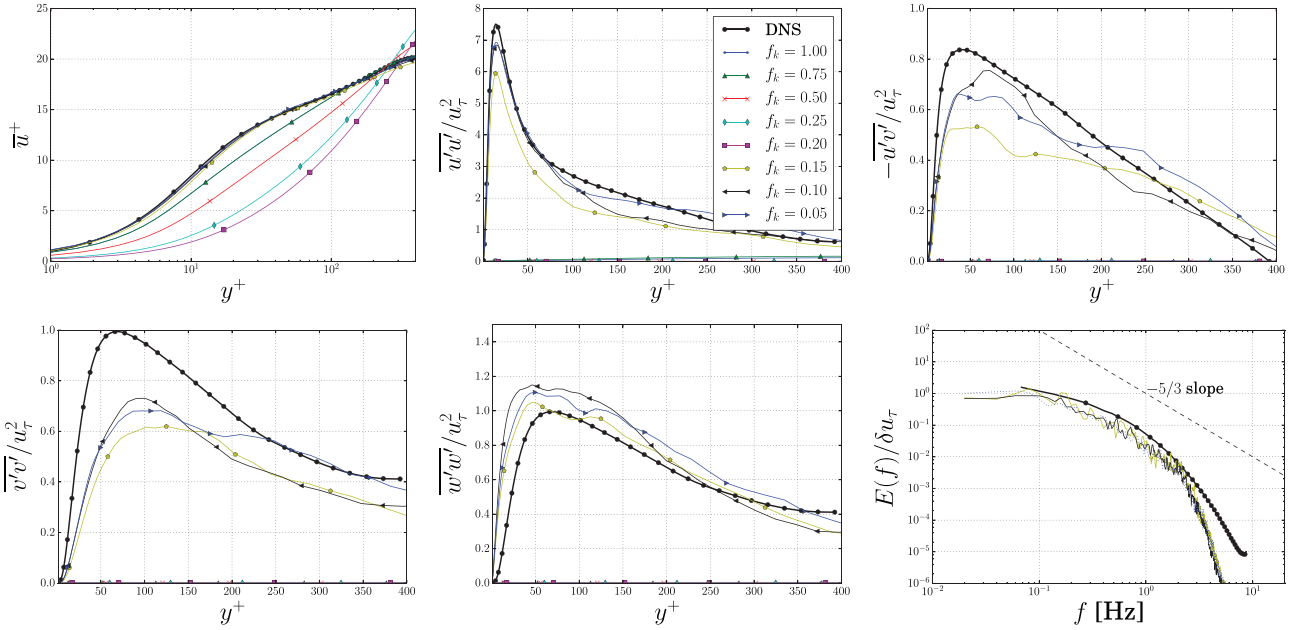
Fig. 12. Normalised mean velocity and Reynolds stress profiles and turbulence kinetic energy spectra using PANS and DNS [28]. From left to right, and top to bottom \bar{u}^+ , Re_{uu} , Re_{uv} , Re_{vv} , Re_{vw} and E_{u,y^+ \approx 20}(f) .
