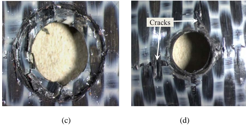
Fig. 16. The Hi-Lok ® collar (HL12V6) after the PT test (a) and the side (b), bottom (c) and top (d) view of fracture surface of bottom adherend after removing the fastener.
