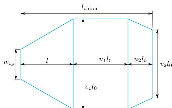
Figure 2 Parametrisation of the cabin floor, note l_{cabin} is not a variable but a result of the parametrisation.
