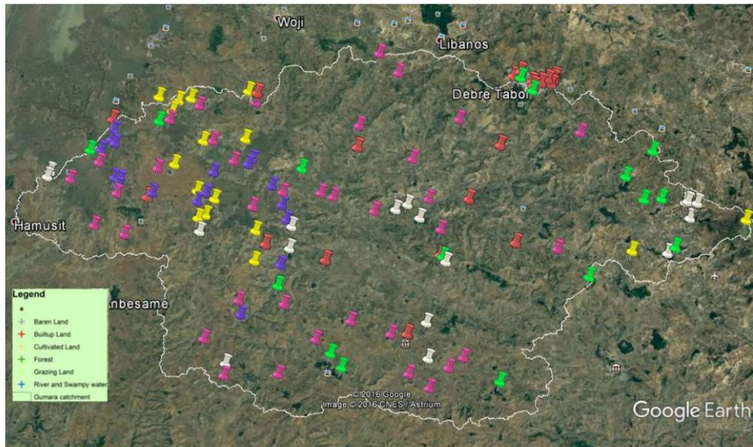
Figure 4: The location of ground truth data points across the Gumara Catchment.
