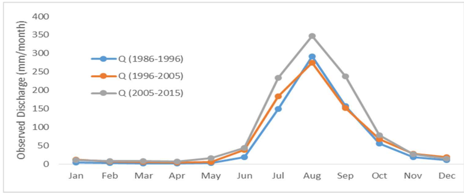
Figure 9: Statistical analyses indicating decadal means of precipitation and observed discharge.
