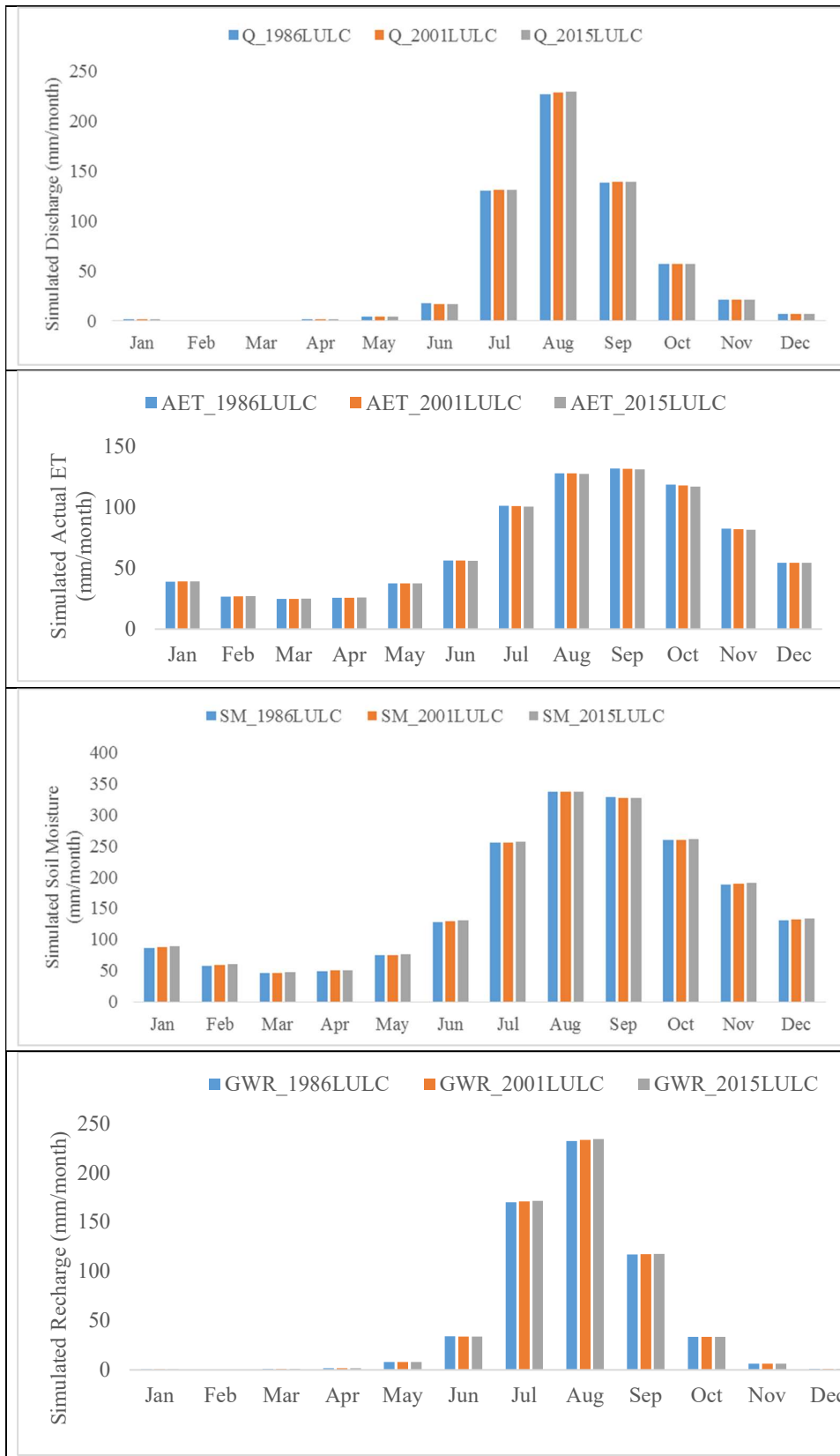
Figure 8: Simulated water balance components under studied LULC scenarios.
