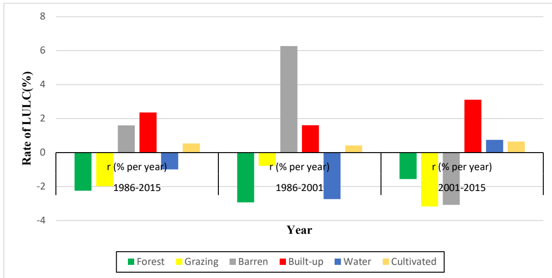
Figure 6: Annual rate of LULC change between 1986 and 2015.
