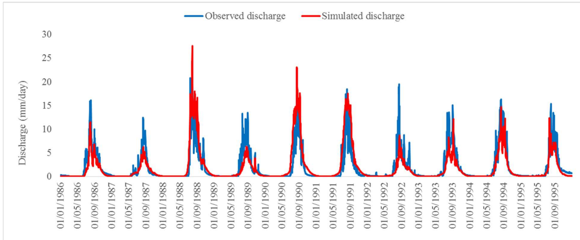
Figure 7: A comparative view of observed and simulated discharge during calibration (1986-1990) and validation (1991-1995).
