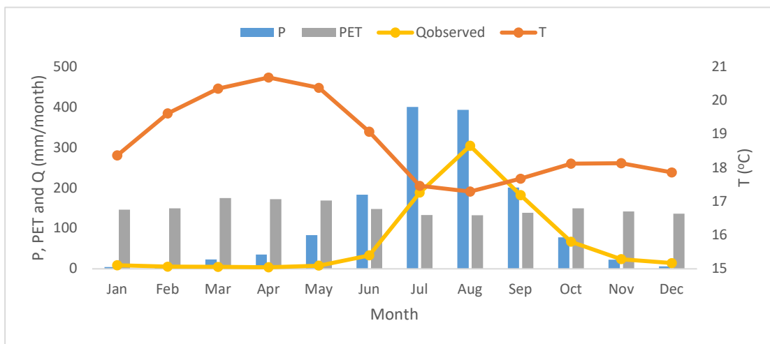
Figure 2. Mean monthly climate and river discharge for the period between 1985 and 2015. P , PET , Q and T refer to precipitation, Potential evapotranspiration, river discharge and temperature, respectively.
