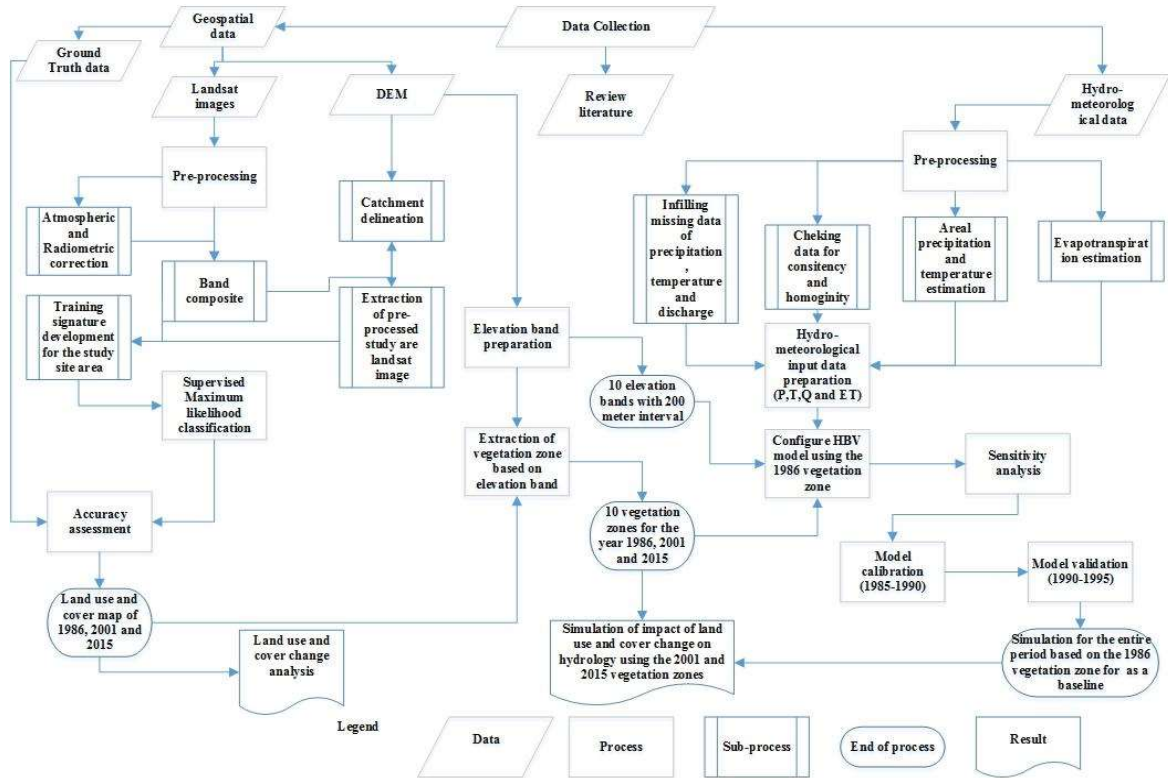
Figure 3: Methodological framework applied for the land use and cover mapping and hydrological modelling.
