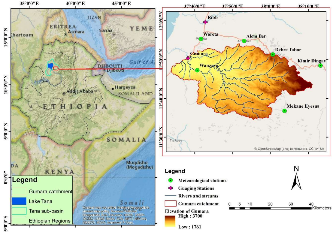
Figure 1: Location of study area and hydro-meteorological stations used for the study.
