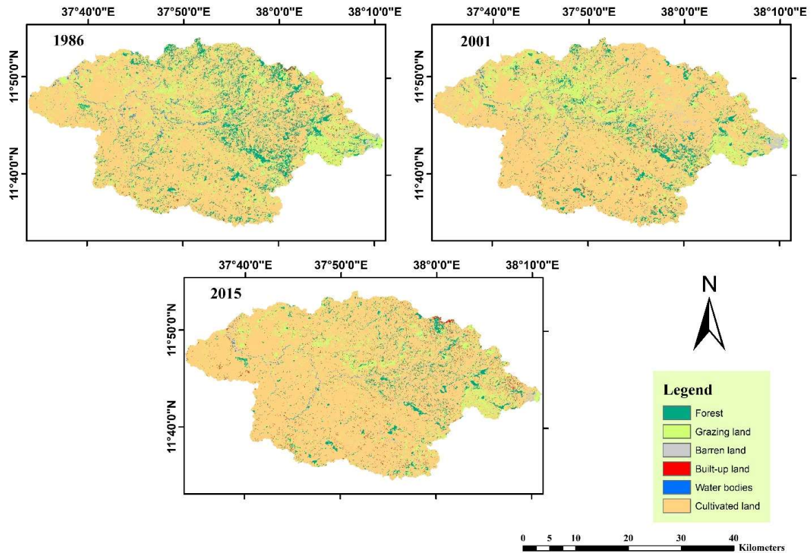
Figure 5: The LULC maps of the Gumara catchment for the year 1986, 2001 and 2015.
