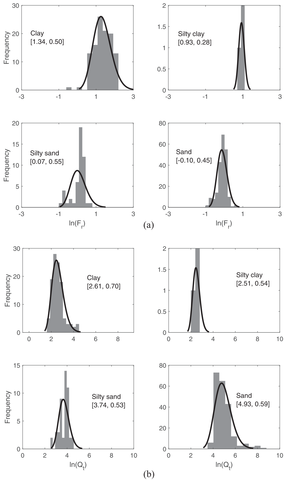
Fig. 9. Histograms of (a) \ln(F_r) and (b) \ln(Q_t) for four soil units obtained from the most likely soil classifications identified at the CPT locations. The values inside square brackets are the means and standard deviations of lognormal distribution fits to the histograms.
