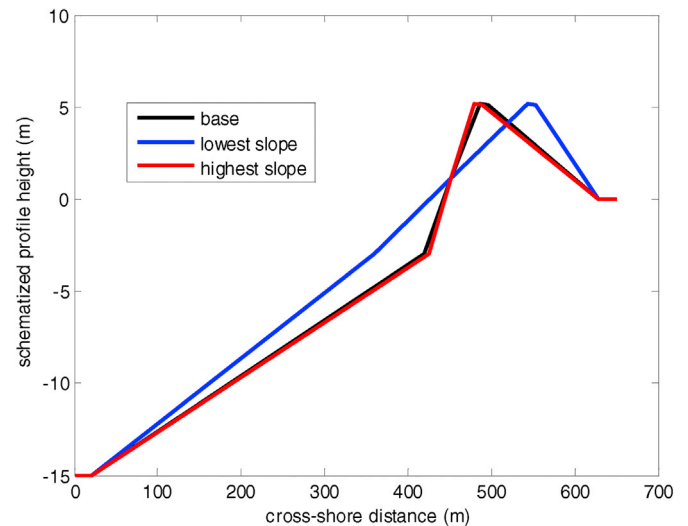
Fig. 11. Base, mildest and steepest profile for simulations.
