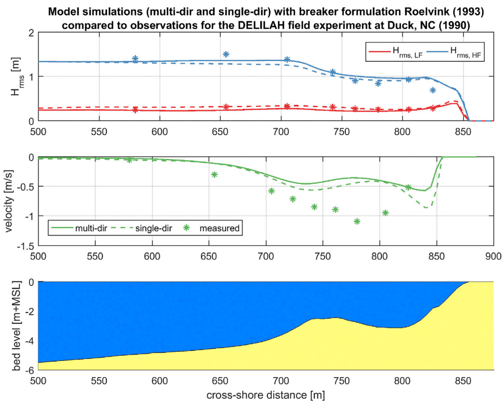
Fig. 7. Top panel: High-frequency (blue) and low-frequency (red) H_{rms} simulated with multi-dir (drawn lines) and single-dir (dashed lines), vs observations indicated by asterisks. Middle panel: comparison for longshore velocity. Bottom panel: bottom profile. Breaker formulation Roelvink (1993). (For interpretation of the references to colour in this figure legend, the reader is referred to the web version of this article.)
