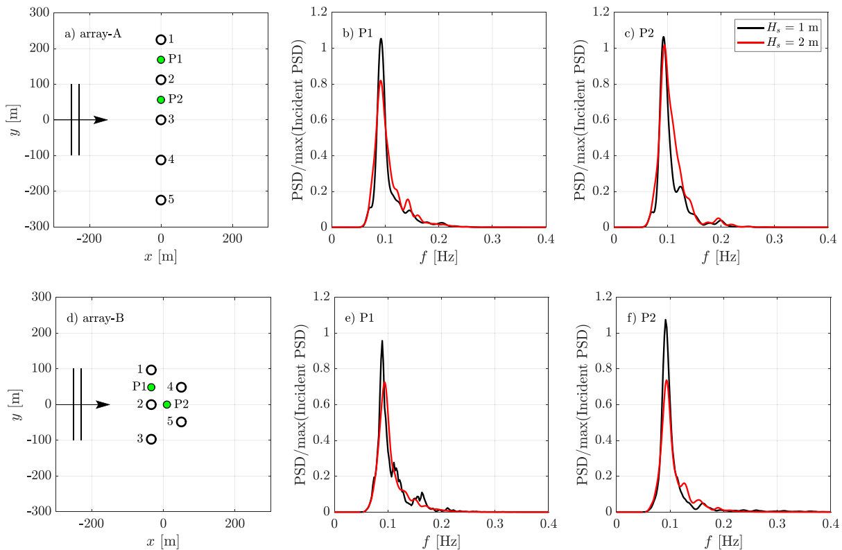
Fig. 18. Comparison of normalized surface elevation spectra from WEC-SWASH at two different locations for the two representative arrays ( H_s = 1 m, 2 m, T_p = 11 s).
