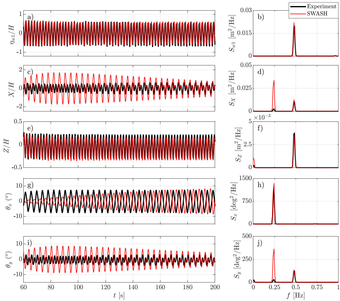
Fig. 8. Comparison of SWASH predicted and experimentally measured time series and power spectral densities (PSDs) subject to H = 0.05 m and T = 2.1 s. Panels (a) and (b) show the normalized time series and PSD of the incident wave. Panels (c), (e), (g) and (i) show the time histories of surge, heave, roll and pitch motions with their PSDs in (d), (f), (h) and (j), respectively.
