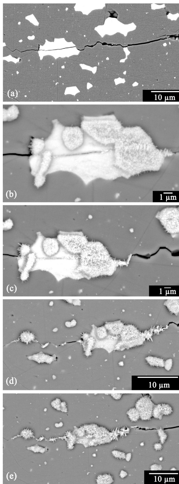
Fig. 10. Evolution of crack-gap filling of another area of the same sample as in Fig. 9. (a) Starting material, (b) Annealed after 1 h, (c) 2 h, (d) 4 h, and (e) 6 h.
