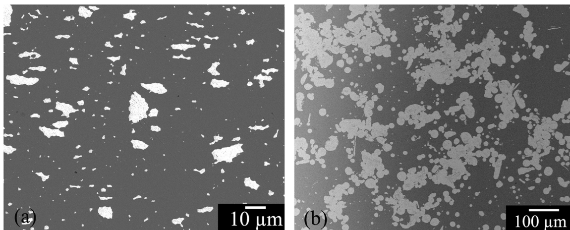
Fig. 2. Microstructure of the Al 2 O 3 Ti composite showing the distribution of Ti (white phase) in alumina produced with (a) and without (b) adding the surfactant Dolapix.
