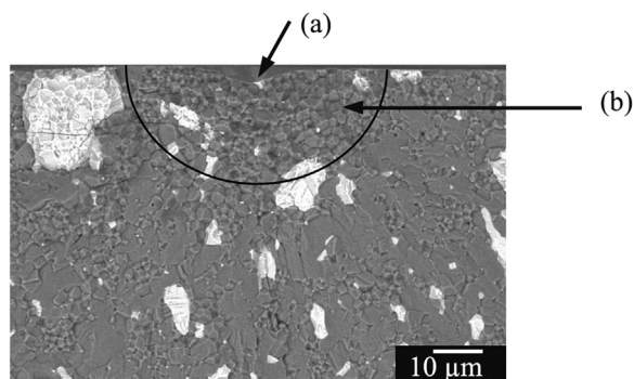
Fig. 6. Cross section of indented surface (a) Marks the imprint of the indenter and (b) The half-penny crack.
