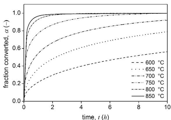
Fig. 3. Fraction of Ti powder converted to TiO 2 α, in dry synthetic air as a function of time t, for different annealing temperatures.
