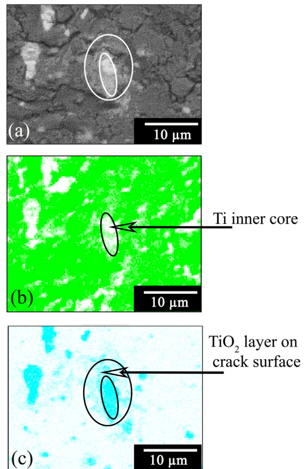
Fig. 13. (a) SEM image of a crack plane after annealing at 800 °C for 30 min in air, (b) O K\alpha X-ray map and (c) Ti K\alpha X-ray map of the same area.
