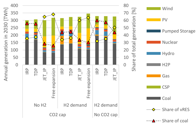
Fig. 4. – Total annual generation and share of chosen technologies in total generation on the secondary axis. vRES: variable renewable energy includes solar, wind and hydro.
