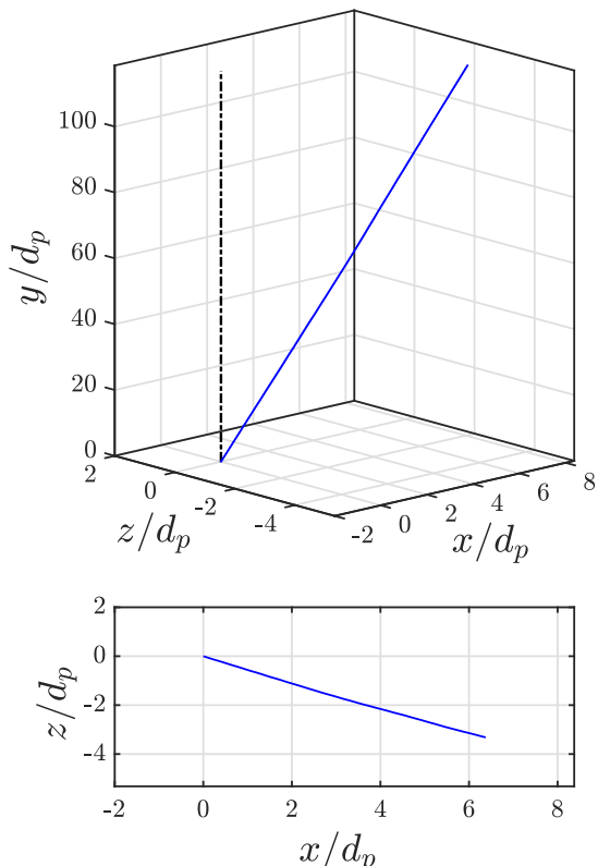
Fig. 17. Steady oblique trajectory for \bar{\rho} = 0.892 and Ga = 159.36 rising at an angle of 3.47^\circ with a mean vertical velocity ( \bar{v}_y/v_g ) and horizontal velocity ( \bar{v}_h/v_g ) of -1.38 and 0.084 , respectively.
