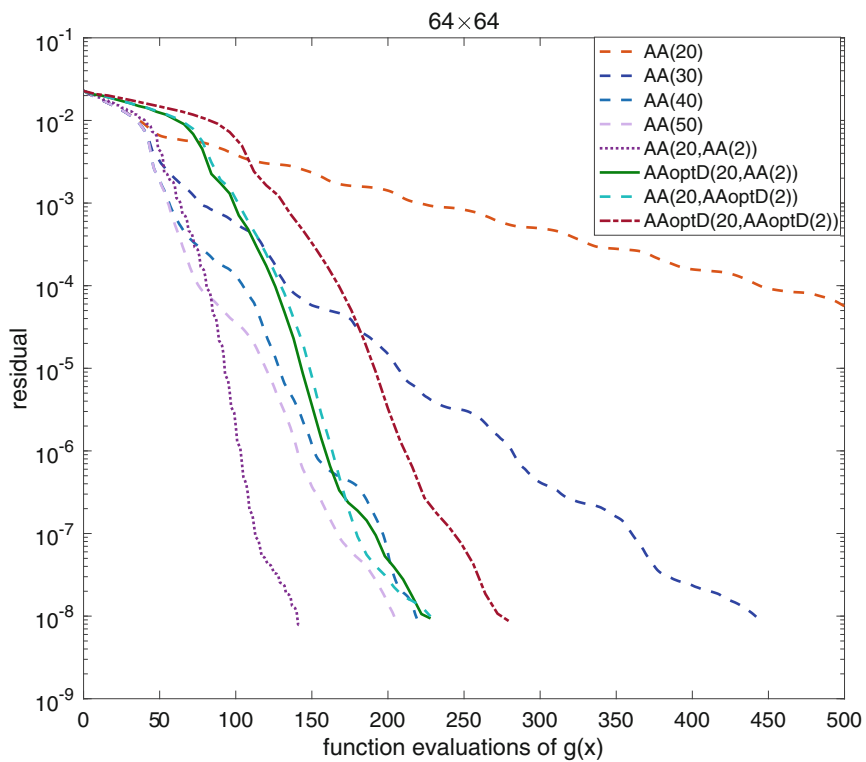
FIGURE 4 Solve the Bratu problem with zero initial approximation, inner loop m = 20 , and outer loop n = 2
