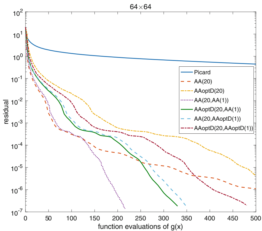
FIGURE 6 Solve the Bratu problem with random initial approximation, inner loop m = 20 , and outer loop n = 1
