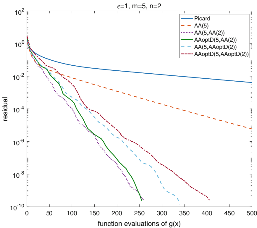
FIGURE 9 Solve the convection-diffusion problem using the central discretization: \epsilon = 1 , larger inner window size
