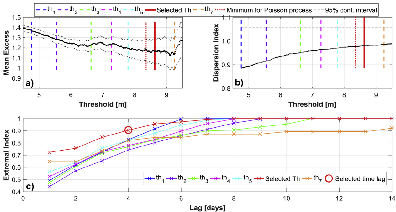
Fig. 5. a), mean residual life plot, 95% confidence intervals based on the approximate normality of sample means, b) dispersion index considering all 7 investigated thresholds and c) extremal index for combination of all seven investigated thresholds and 14 declustering time lags.
