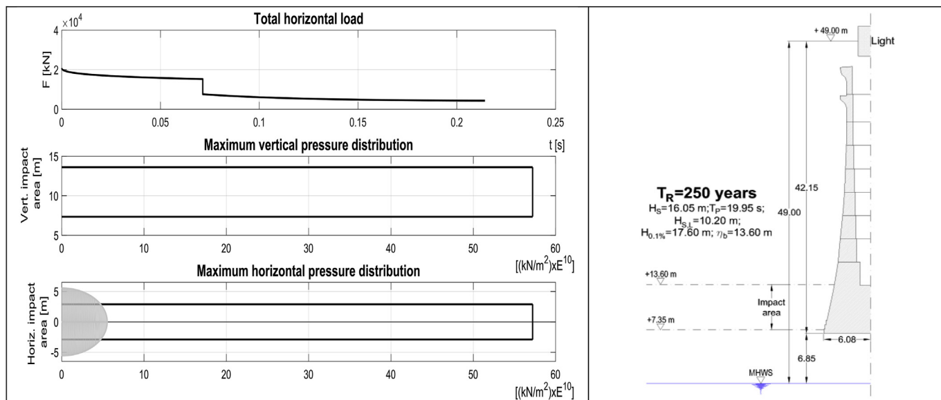
Fig. 13. 250 year wave breaking load. Left upper panel: total load time series; left central panel: vertical pressure distribution; left bottom panel, horizontal pressure distribution. Right panel: impact area.
