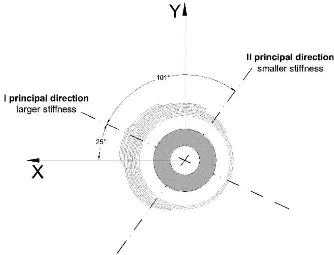
Fig. 17. Top view of the lighthouse. Accelerometers alignments (X and Y) and identified principal directions.
