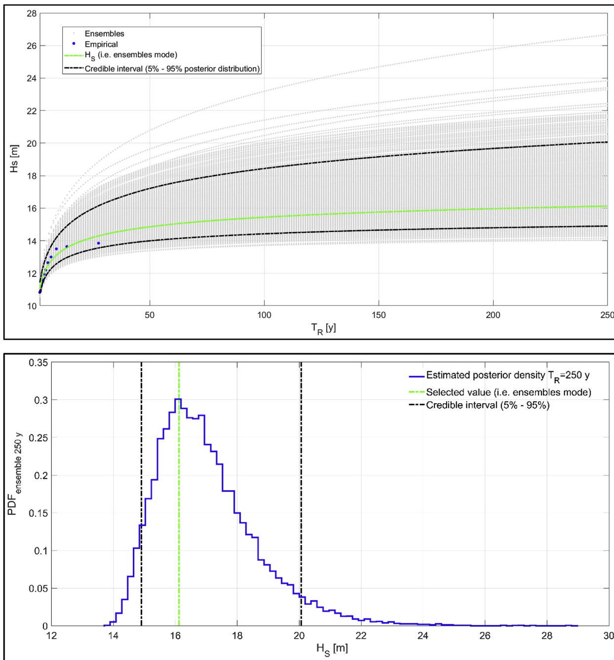
Fig. 10. Upper panel, identified design values and related credible interval. Lower panel, posterior density distribution for return level equal to 250 years.
