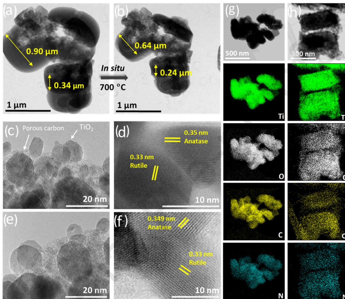
Fig. 2. (a) STEM image of as-prepared \text{NH}_2\text{-MIL-125(Ti)} and (b) after in-situ heating under \text{N}_2 gas atmosphere up to 700 °C. The shrinkage of particle size ( \sim 30\% volume) can be observed with the preserved morphology and porosity. The HRTEM images of (c, d) \text{N-C-TiO}_2/\text{C}_{\text{Ar}} and (e, f) \text{N-C-TiO}_2/\text{C}_{\text{ArW}} . EDX elemental mappings of (g) \text{N-C-TiO}_2/\text{C}_{\text{Ar}} and (h) \text{N-C-TiO}_2/\text{C}_{\text{ArW}} respectively.
