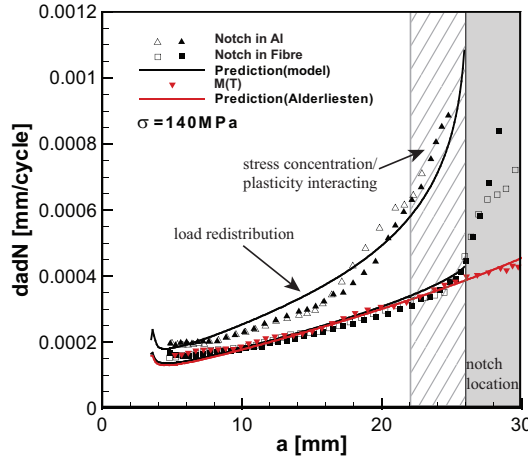
Figure 2.9: Comparison between predicted and experimental crack growth rate for Glare 3-3/2 with notches in Al layers or fibre layers with \sigma_{max} = 140MPa
