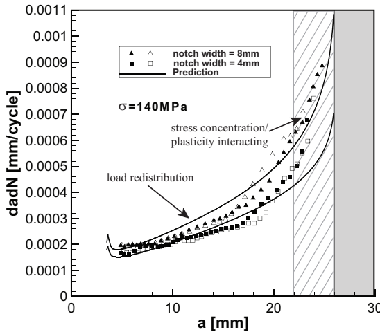
Figure 2.10: Crack growth rates for Glare 3-3/2 panels with different notches of 8mm and 4mm wide in Al layers under \sigma_{max} = 140MPa
