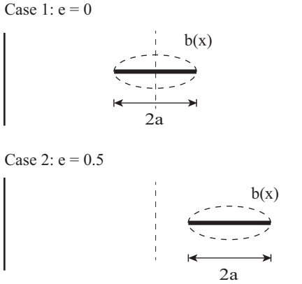
Figure 3.12: Illustration of two crack cases
