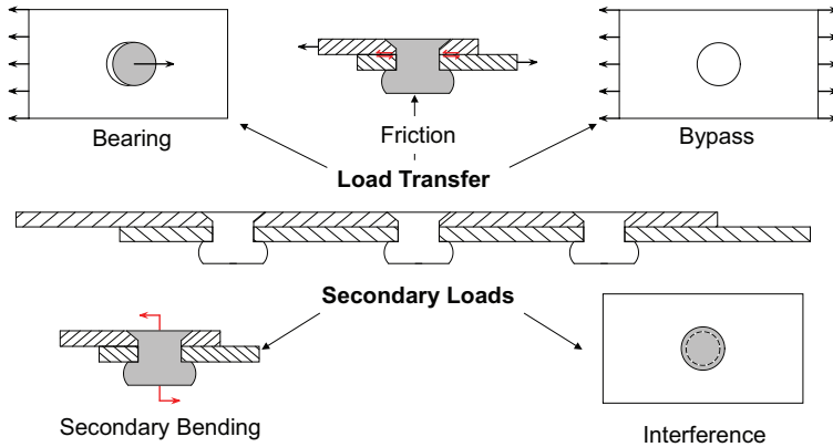
Figure 7.2: Loading components in a mechanically fastened joint [1]
