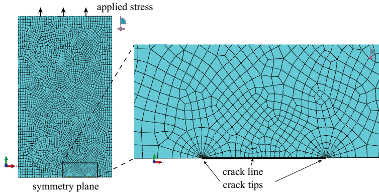
Figure 3.8: Mesh of the FEA model for an Al 2024-T3 panel with an eccentric crack
