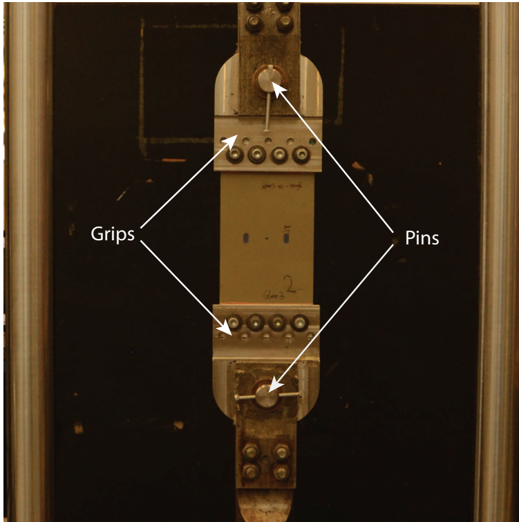
Figure 2.7: Test set-up
