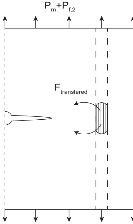
Figure 2.4: Illustration of load redistribution due to notch
