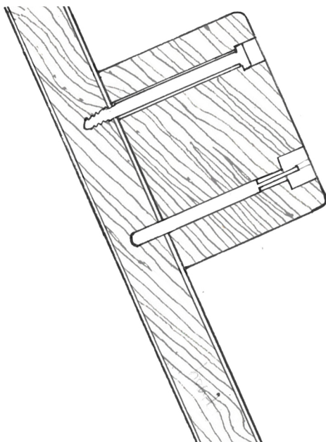
Wall-wall hook longitudinal and frontview
