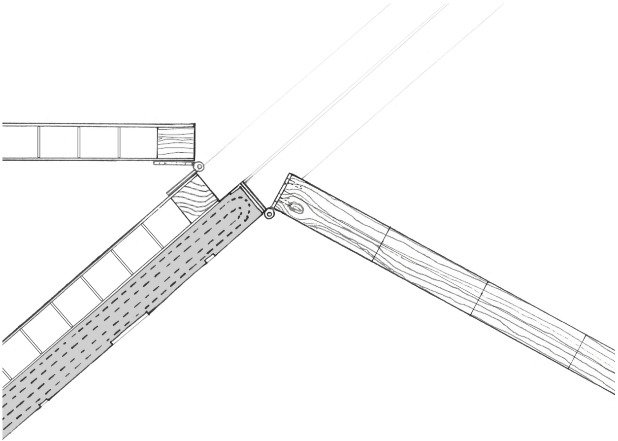
Door hinge connection longitudinal
