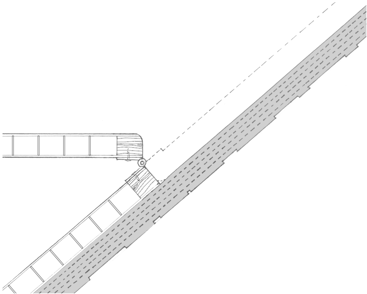
Floor hinge connection longitudinal
