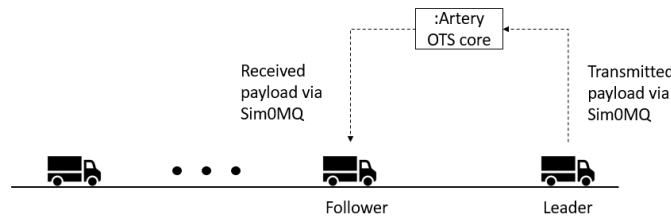
Figure 1: OTS-Artery architecture showing information exchange between a leader-
