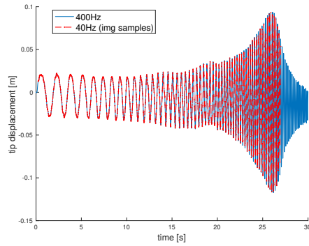
(b) Sweep signal: \alpha_g = 5^\circ , f_g = 0.1 - 10 Hz, V = 30 m/s.
