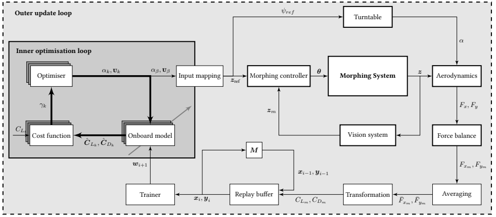
Figure III.3.6: Online shape optimisation architecture diagram with inner optimisation loop and the corresponding components marked in dark gray.
