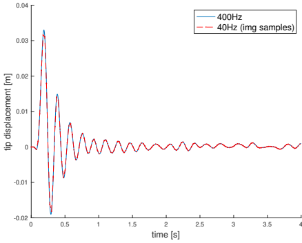
(a) Gust signal (1-cos): \alpha_g = 10^\circ , f_g = 5 Hz, V = 30 m/s.
