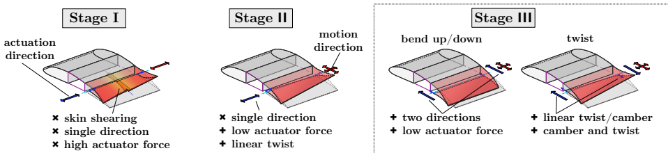
Figure II.1.2: TRIC morphing concept design evolution stages I-III by Werter et al. [29].
