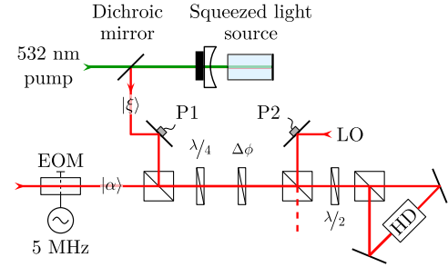
Fig. 3. Experimental implementation. A vacuum squeezed state, created by parametric downconversion, and a coherent state, generated by an electro-optic modulator (EOM), are sent into a polarization-based Mach-Zehnder interferometer (MZI). A quarter-wave plate in combination with a motorized half-wave plate ( \Delta\phi ) forms the equivalent phase shift of a MZI where the two modes are spatially separated. The piezo transducers P1 and P2 stabilize the phase between the input states and the local oscillator (LO), respectively. A half-wave plate in front of the last polarizing beam splitter is used to balance the photocurrent in the homodyne detector (HD). All cubes represent polarizing beam splitters.
