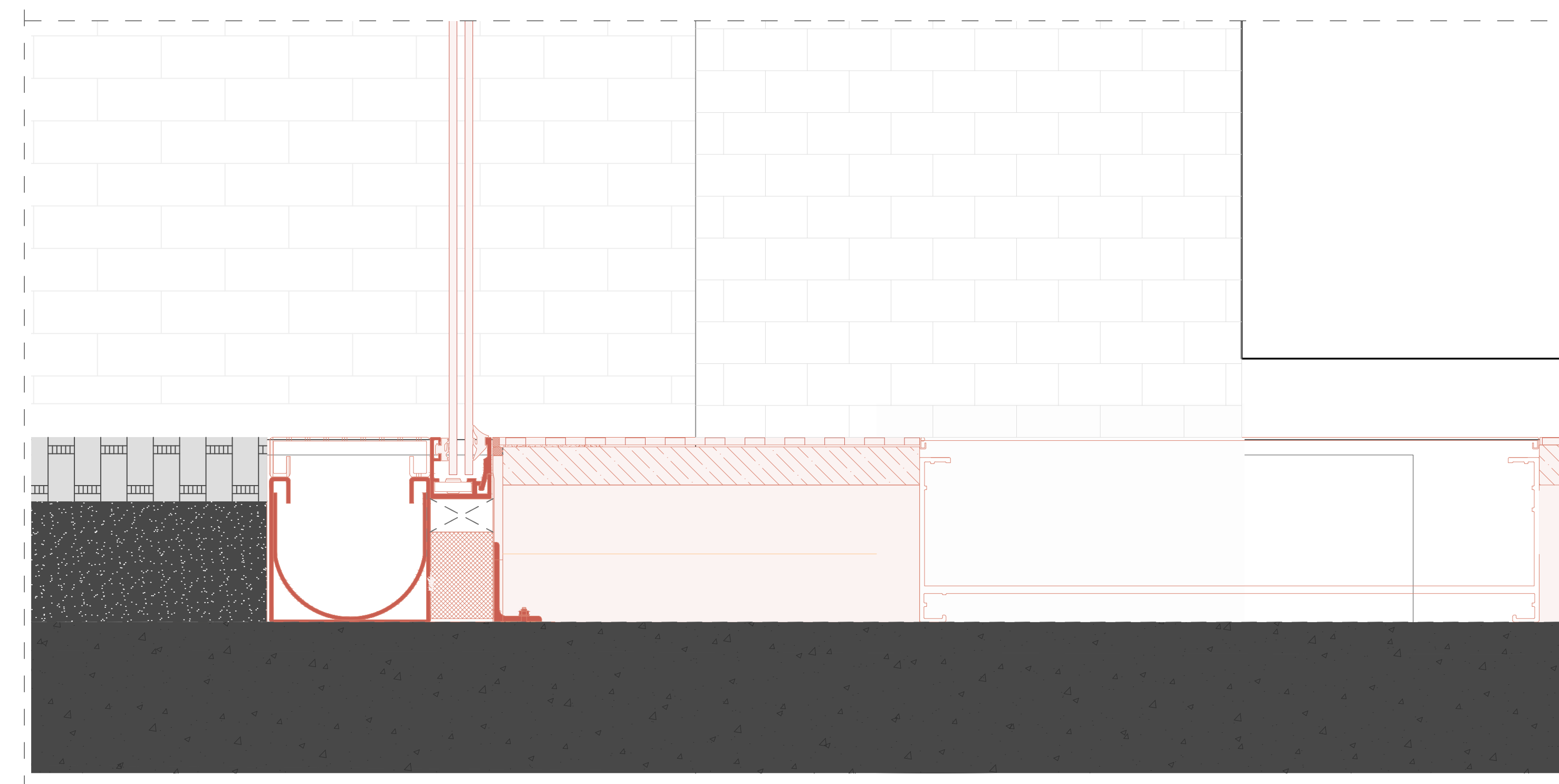
Detail 1:5 sunken sill with drainage
