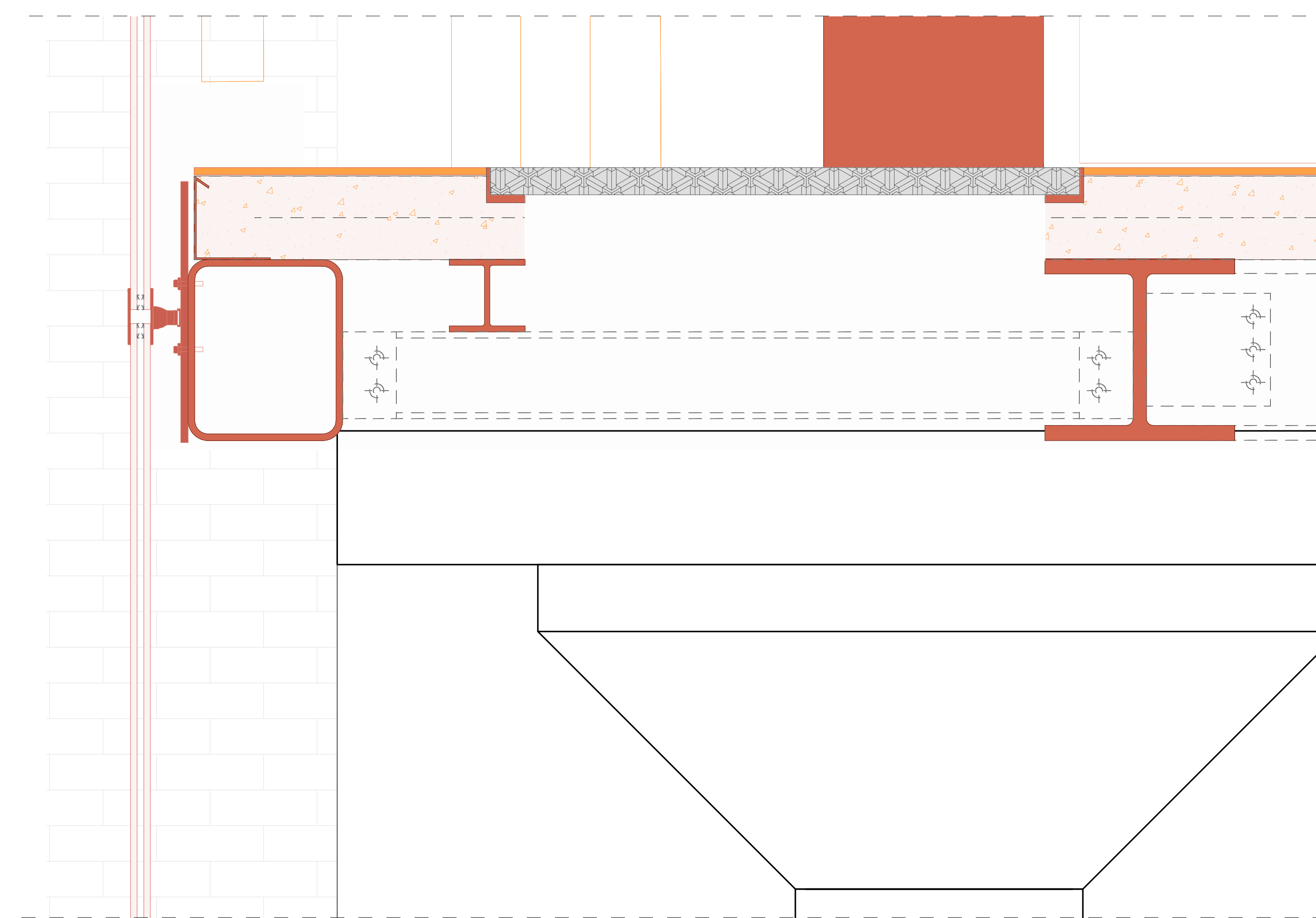
Detail 1:5 curtain wall point support fixing
