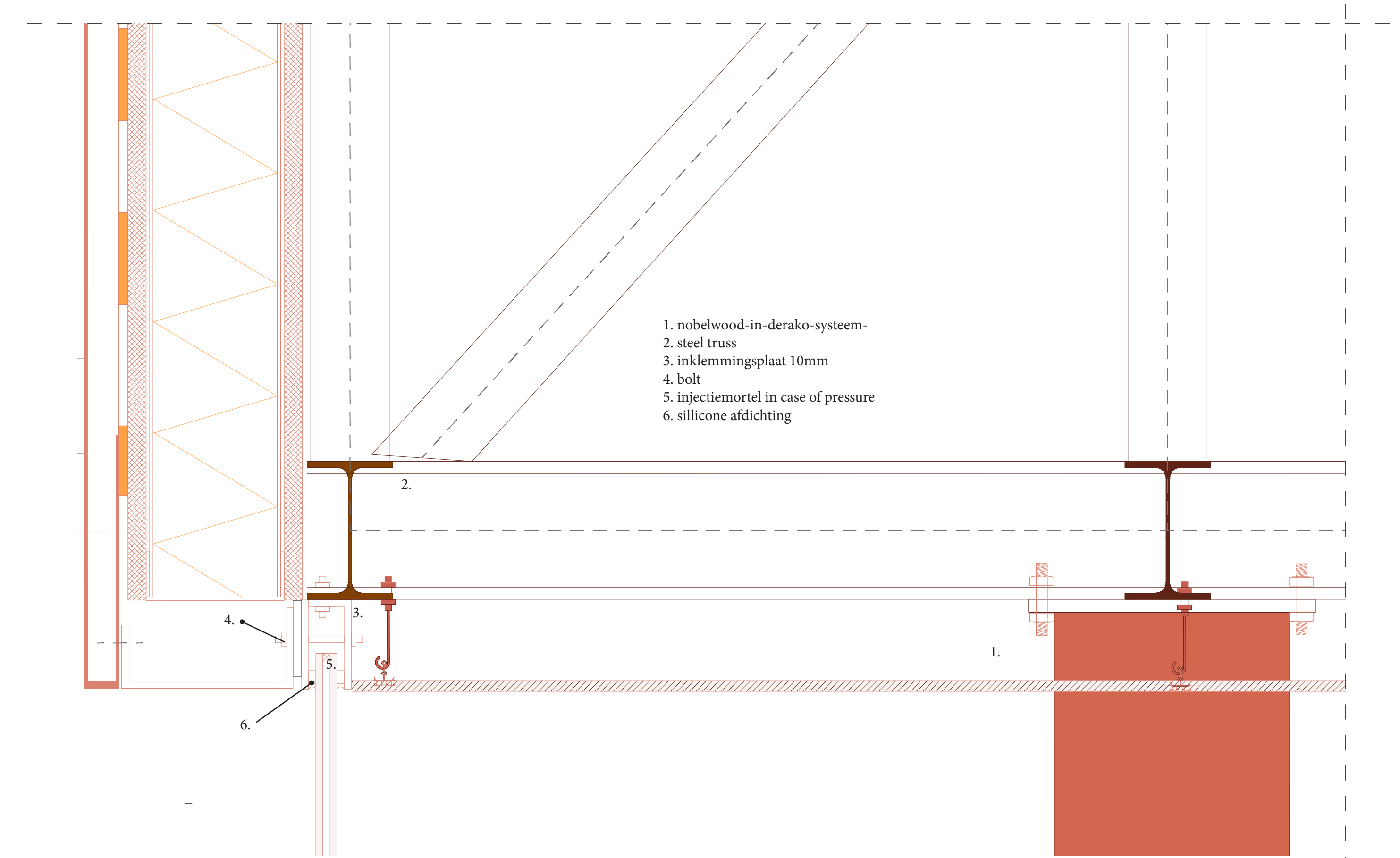
Detail 1:5 curtain wall point support fixing
