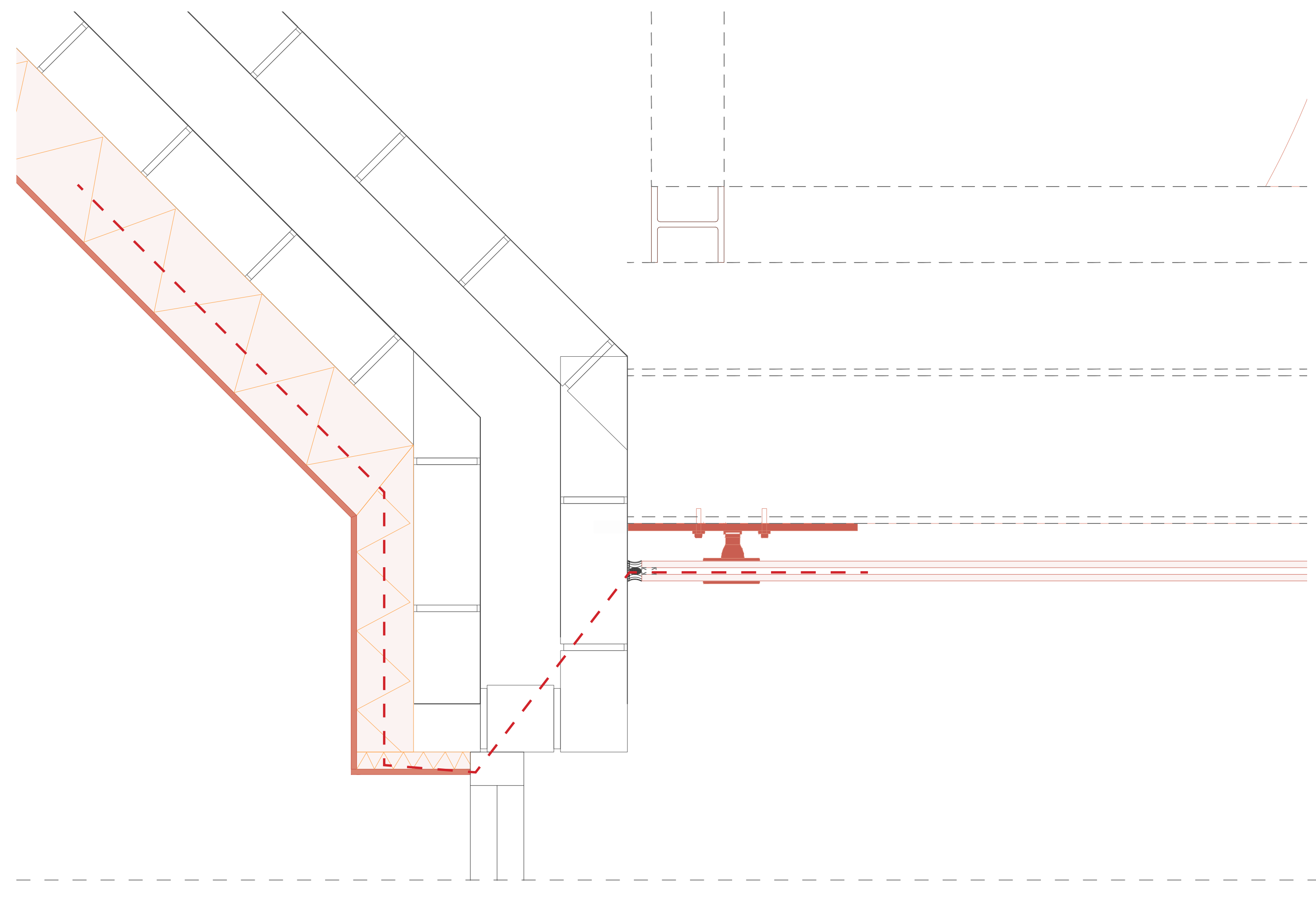
Detail 1:5 curtain wall connection to existing building
