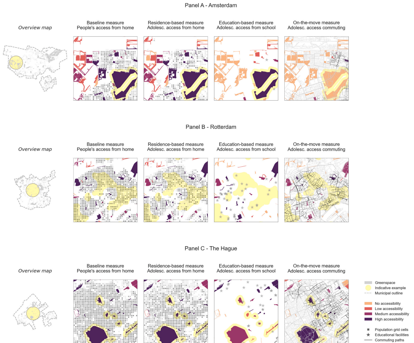
Fig. 3. Adolescents' greenspace accessibility: baseline, residential, educational and on-the-move accessibility measures for Amsterdam (A), Rotterdam (B) and The Hague (C). Notable examples are highlighted in yellow. (For interpretation of the references to colour in this figure legend, the reader is referred to the web version of this article.)
