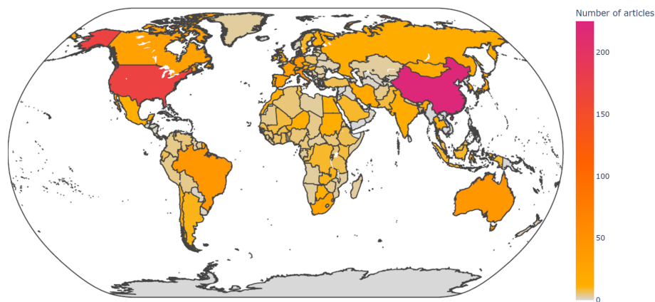
Figure 11. Number of articles per country where uncertainties in RS-ET were assessed.
