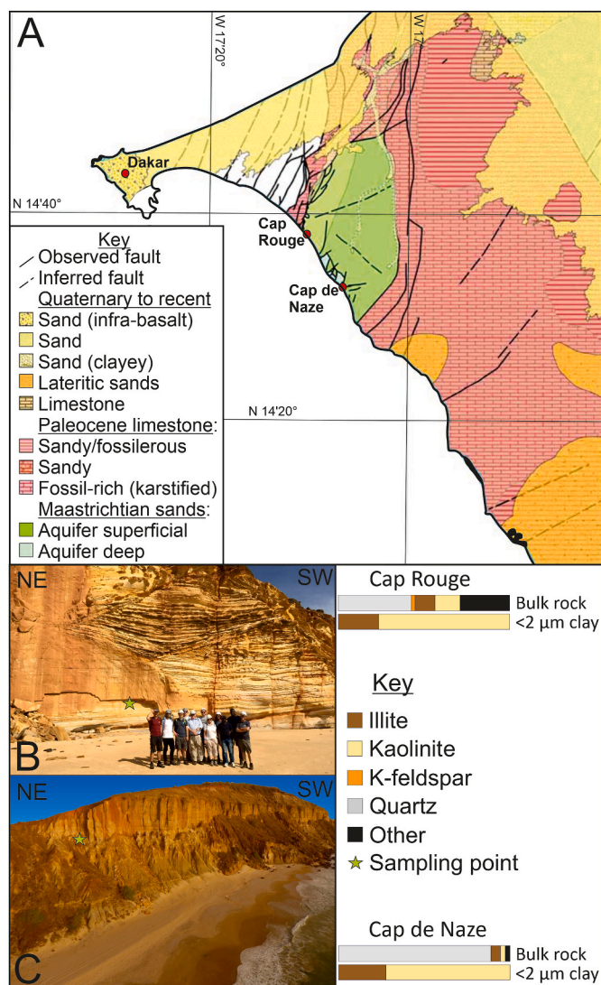
Fig. 9. A, Geological map of western Senegal (M'bour region) modified from Barousseau et al. (2009). B, Cap Rouge exposure and associated bulk rock and <2 \mu\text{m} clay mineralogy. C, Cap de Naze exposure and associated bulk rock and <2 \mu\text{m} clay mineralogy.
