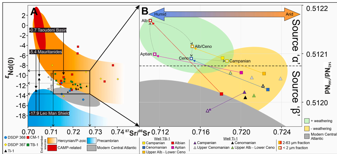
Fig. 6. A, Cross plots of \epsilon_{Nd}(0) and ^{87}Sr/^{86}Sr values, DSDP367, 368 and CM-1 taken from Mourlot et al. (2018 2 ) and TB-1 and Ti-1 from this study. Highlighted in black are average \epsilon_{Nd}(0) values for the three most proximal NW-African sources to the MSGBC Basin (Taoudeni Basin, Mauritanides and Leo Man Shield) established by Mourlot et al. (2018 2 ). B, Magnification of Fig. 6A; ^{143}Nd/^{144}Nd and ^{87}Sr/^{86}Sr values for samples from TB-1 and Ti-1 including < 2 \mu m and 2–63 \mu m fractions, “orange” Hercynian/Palaeozoic source divided into source \alpha (green) and source \beta (yellow).
