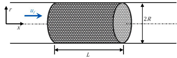
Figure 7. Physical model and coordinate system, adapted from Singh, et al. (2006).
