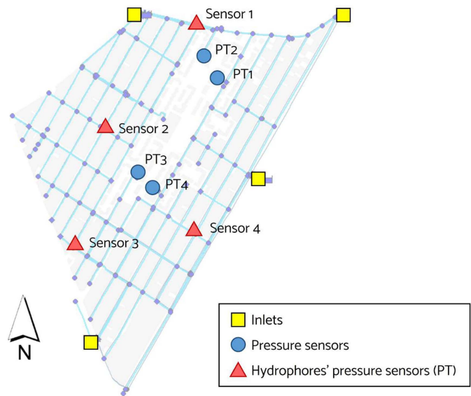
Fig. 3. Sensors' placement in the case study.
