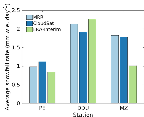
Figure 8. Daily average snowfall amounts ( \text{mm w.e. day}^{-1} ) for the concurrent periods displayed in Fig. 2 for the Princess Elisabeth (PE), Dumont D’Urville (DDU) and Mario Zucchelli (MZ) stations. CloudSat snowfall amounts are derived for the grid specified by Palermé et al. (2014).
