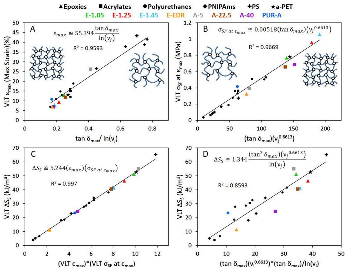
Fig. 3. Plots of VLT (A) strain ( \epsilon_{max} ), (B) stress ( \sigma_{SF} at \epsilon_{max} ), and (D) stored entropic energy density ( \Delta S_S ) from DMA experiments as functions of junction density ( \nu_j ) and \tan \delta_{max} . (C) Calculated VLT \Delta S_S plotted against measured VLT strain ( \epsilon_{max} ) and stress ( \sigma_{SF} at \epsilon_{max} ) from the DMA experiments. Data points in black come from previous studies [41] while A-5, A-22.5, A-40, E-1.05, E-1.25, E-1.45, E-EDR, and PUR-A are identified in colors indicated in the legend above the plots. (For interpretation of the references to color in this figure legend, the reader is referred to the Web version of this article.)
