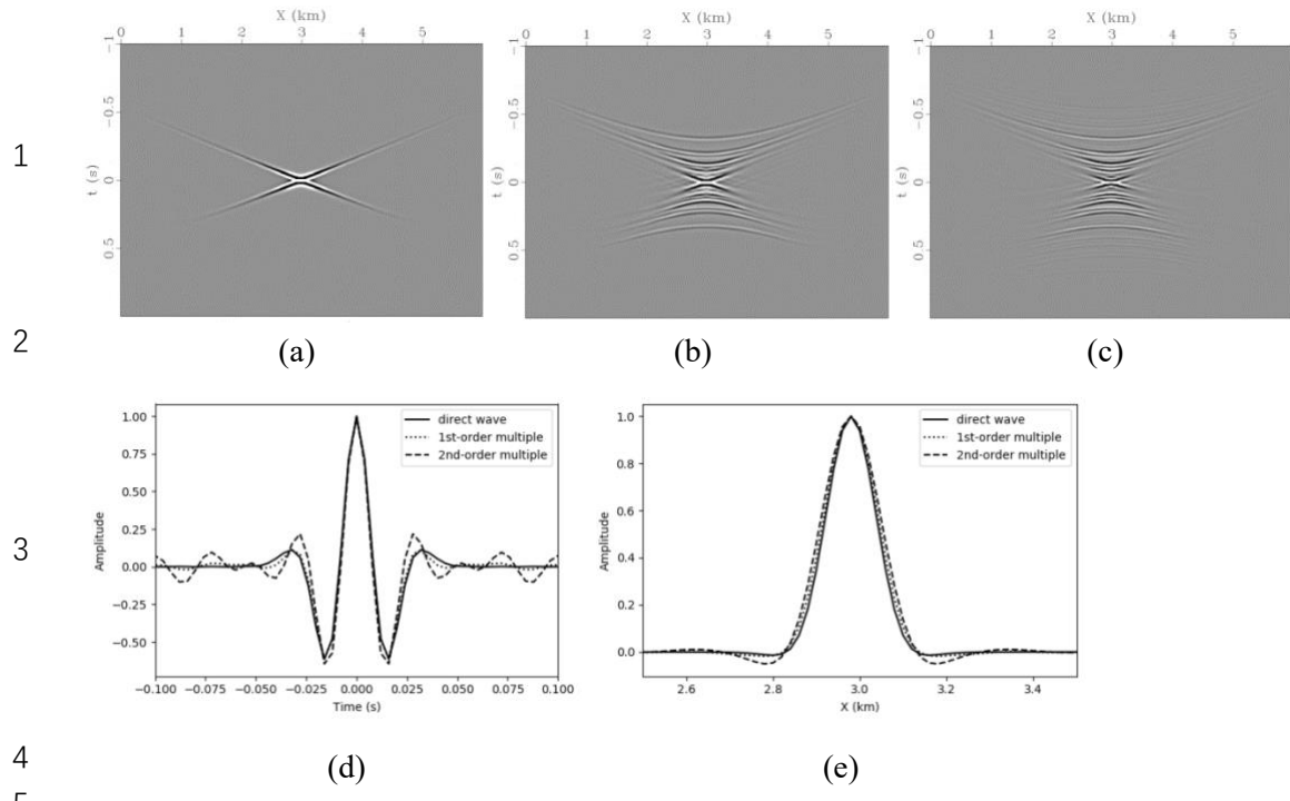
Figure 4: Open-loop Focal beams in a 3D layered model for (a) the direct wavefield, (b) first-order multiple wavefield and (c) second-order multiple wavefield and the slices along the t- (d) and x- (e) directions.
