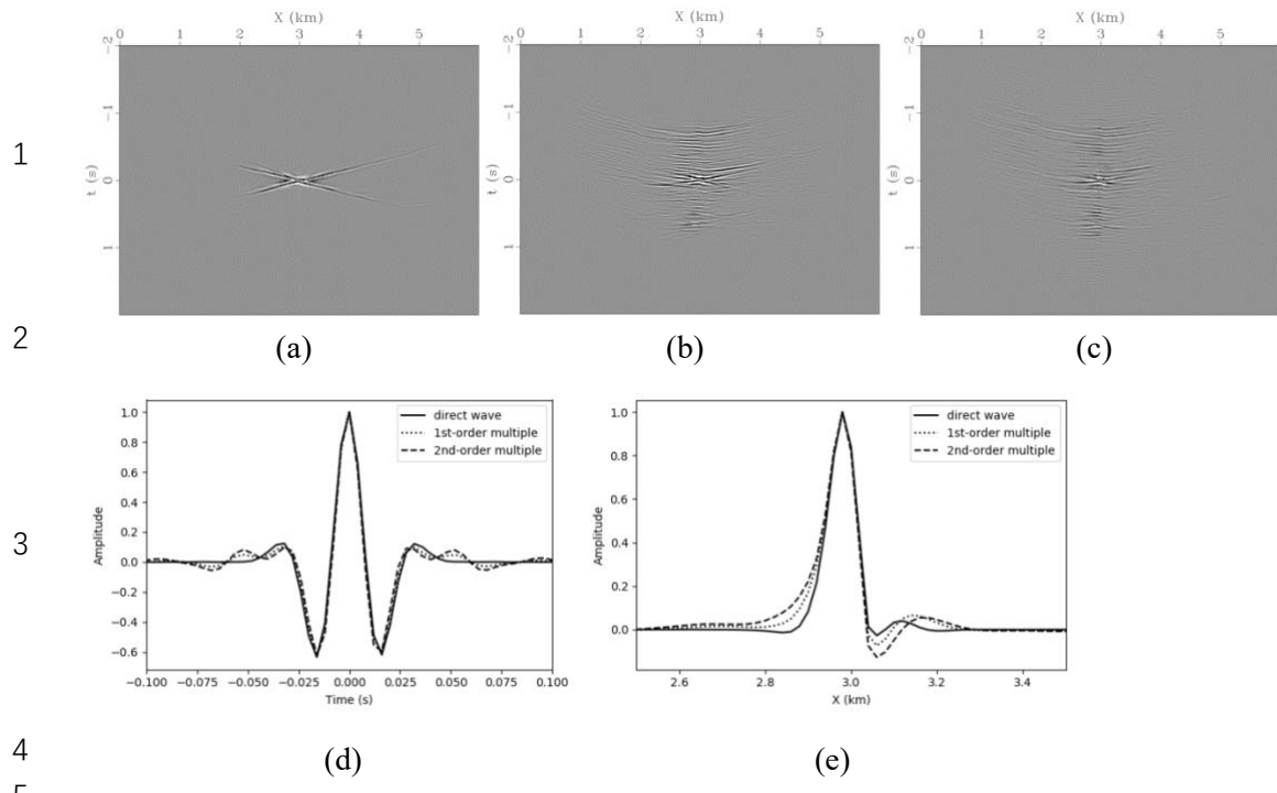
Figure 5: Open-loop Focal beams in a 3D SEG/EAGE salt dome model for (a) the direct wavefield, (b) first-order multiple wavefield and (c) second-order multiple wavefield and the slices along the t - (d) and x - (e) directions.
