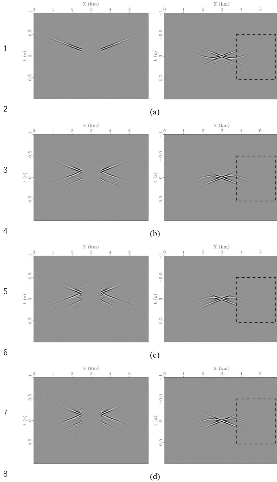
8 9 Figure 8: Open-loop (a) and closed-loop focal operators (left) and beams (right) in a 3D 10 layered model with the maximum order of multiples being 0 (b), 1 (c) and 2 (d). The dashed 11 rectangles mark the difference of migration noise among beams.
