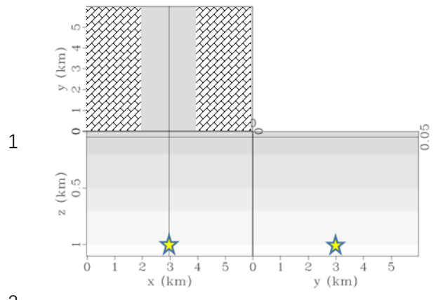
2 Figure 7: The 3D layered velocity model is shown with the gapped source sampling marked 3 by the brick shading. The stars indicate to the target location.
