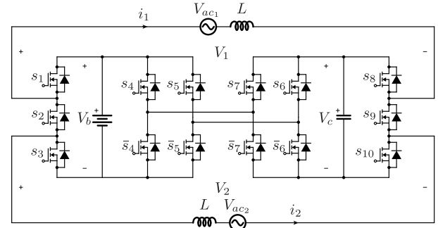
Fig. 1. Proposed dual-output multilevel converter.
