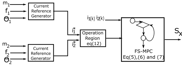
Fig. 2. Model predictive control scheme.
