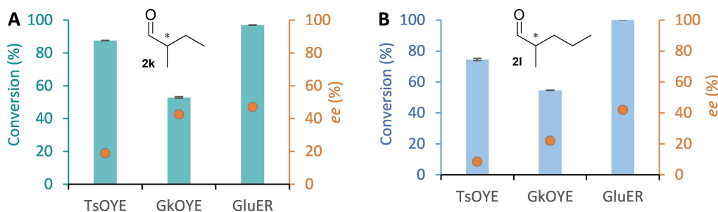
Figure 3. Conversion of unsaturated aldehydes 1k and 1l by TsOYE , GkOYE and GluER after 1 h with BNAH. Brown circles show ee. Conditions: 1 \mu M TsOYE or GkOYE or GluER , 10 mM substrate 1 , 15 mM BNAH, 10% v/v DMSO, 1 mL volume in 50 mM Tris-HCl buffer pH 8.0. (A) trans -2-methylbutenal 1k ; (B) trans -2-methylpentenal 1l .
