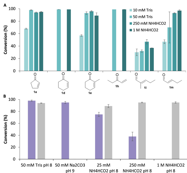
Figure 2. (A) TsOYE -catalyzed reduction of unsaturated ketones and aldehyde substrates 1 after 1 h with BNAH. Conditions: 2 \mu M TsOYE , 10 mM alkene substrate 1 , 15 mM BNAH, 10% v/v DMSO, 1 mL volume. 1d and 1h were tested in 50 mM Tris-HCl and 1 M \text{NH}_4\text{HCO}_2 only. Average of duplicates. (B) TsOYE -catalyzed asymmetric reduction of 2-methylcyclohexenone after 1 h using GDH-recycled NADPH (in purple) or BNAH (in grey). Conditions: 1% v/v DMSO, 2 \mu M TsOYE , 10 mM 2-methylcyclohexenone in different buffer conditions, 1 mL volume. Average of duplicates. purple : with GDH cofactor recycling system: 175 U/mL GDH-105, 0.1 mM NADPH, 12 mM glucose. grey : with 11 mM BNAH cofactor.
