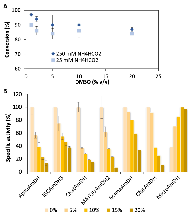
Figure 4. (A) TsOYE -catalyzed reduction of 2-methylcyclohexenone to 2-methylcyclohexanone with 0–20% v/v DMSO after 1 h. Conditions: 2 \mu M TsOYE , 10 mM substrate, 11 mM BNAH cofactor. Average of duplicates. (B) Specific activities of AmDHs for substrate 2j in the presence of 0, 5, 10, 15 and 20% v/v DMSO. For each AmDHs, their maximum specific activity was set up at 100%, which corresponds to specific activity without co-solvent for ApauAmDH , IGCAmDH5 , ChatAmDH , MATOUAmDH2 , MsmeAmDH and CfusAmDH , and to specific activity with 15% DMSO for MicroAmDH . Conditions: 5 mM substrate ( 2j for ApauAmDH , IGCAmDH5 , ChatAmDH and 2d for MATOUAmDH2 , MsmeAmDH , CfusAmDH and MicroAmDH ), 0.04–0.10 mg/mL purified AmDH, 0.4 mM NADH (NADPH for MATOUAmDH2 ) in 1 M ammonium formate buffer pH 9.0 at room temperature (20 °C) ( ApauAmDH , MsmeAmDH , CfusAmDH , MicroAmDH ) or 50 °C ( IGCAmDH5 , MATOUAmDH2 , ChatAmDH ). Specific activities were calculated based on spectrophotometric assay (see SI for details). Errors bars represent the standard deviation of two independent experiments.
