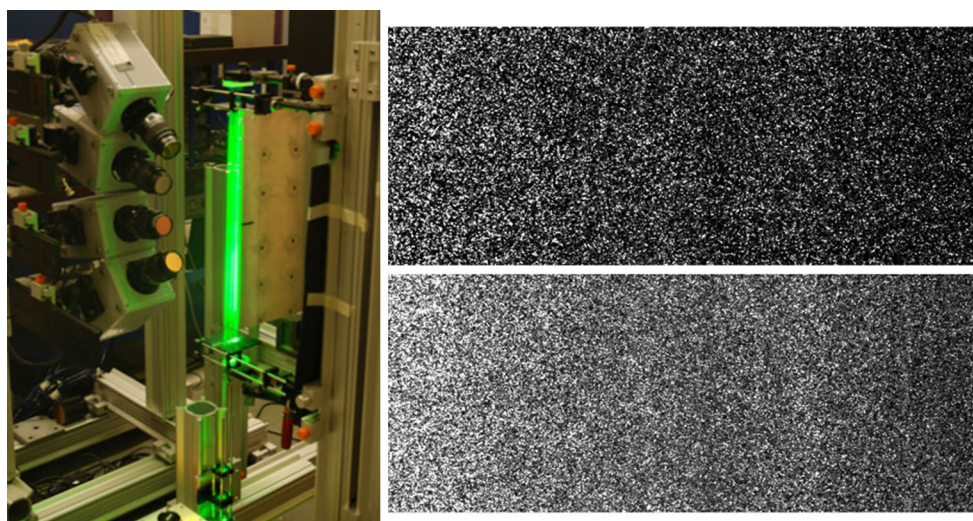
Fig. 8 Left tomographic PIV setup (reproduced from Ghaemi and Scarano 2011). Right individual particle images after preprocessing (cropped to 500 \times 200 pixels) at \text{ppp} = 0.05 (top) and 0.2 (bottom)
