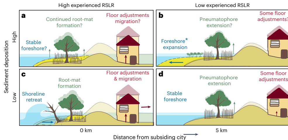
Fig. 5 | A summarizing schematic representation of the key processes affecting cross-shore profiles under low and high RSLR rates (columns), in the presence of low and high sediment availability (rows). The transparent profiles in the background represent pre-subsidence profiles. The solid lines and figures represent sunken profiles. Sea level rise is represented by the translucent water level above the blue water level. The dashed lines represent sedimentation (yellow) or erosion (transparent (only in c)). c and d are based on situations as we have observed at our study site at 0 km and 5 km from the subsiding city. a and b are hypothetical scenarios and expected effects based on literature (*). a, Vegetated foreshores are expected to remain stable if the sediment availability matches RSLR at the foreshore 5 . Trees may survive RSLR and sedimentation rates by forming new root mats in freshly deposited sediment, but long-term survival under these conditions is unsure. Under these conditions, migration of people
