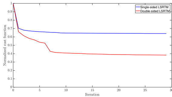
Figure 3.9.: Cost function comparison of homogeneous background velocity case.
