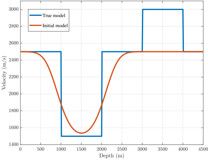
Figure A.1.: True and initial model
