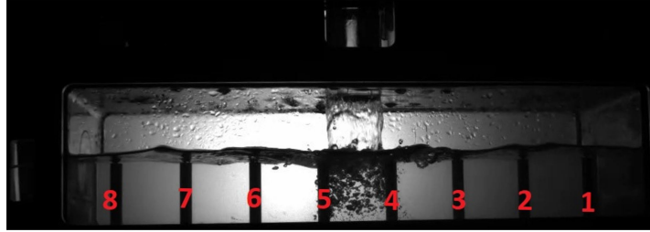
FIG. 16: Horizontal header and vertical downward channels, central vertical inlet of 56-mm I.D. and a channel intrusion of 1/2 of the header height
