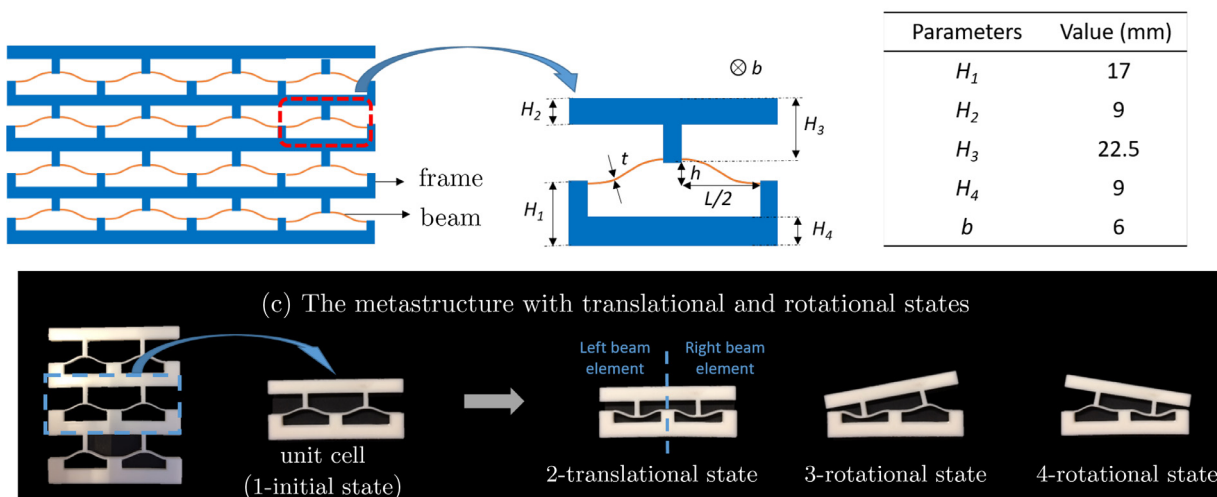
Fig. 1. A demonstration of multi-stable structures with translational and rotational stable states. (a) A schematic for the proposed multi-stable metastructure. The structure is designed by serially stacking curved beams with thick frames. (b) Geometric parameters of the beam element are depicted. The out-of-plane dimension is denoted as b . (c) Each unit cell ( h = 5 mm t = 0.8 mm and L = 28 mm) possesses four stable states such that it can snap into the translational state or the rotational states.
