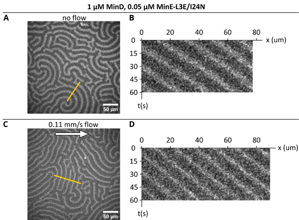
Fig. C1 | Min patterns for 1 \mu\text{M} MinD + 0.05 \mu\text{M} MinE-L3E/I24N. The Left shows a single frame; the right shows kymographs that were taken at the yellow line indicated on the left. A Snapshot of the pattern without flow. B Kymograph of designated line trace without flow. C Snapshot of pattern with 0.11 mm/s bulk flow. D
