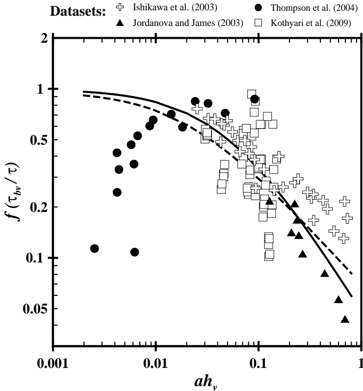
Figure 5.9: Emergent artificial vegetation: ratio between bed-shear stress and total shear stress for vegetated beds as a function of ah_v . Measured values against estimated by Baptiste (2005) (Continuous line), and Ishikawa et al. (2003) (Dashed line).
