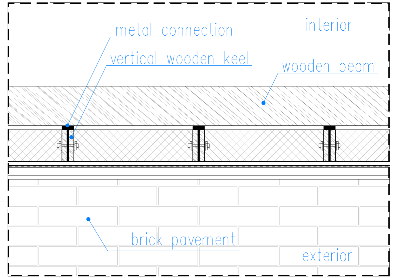
Horizontal section of the new wall
