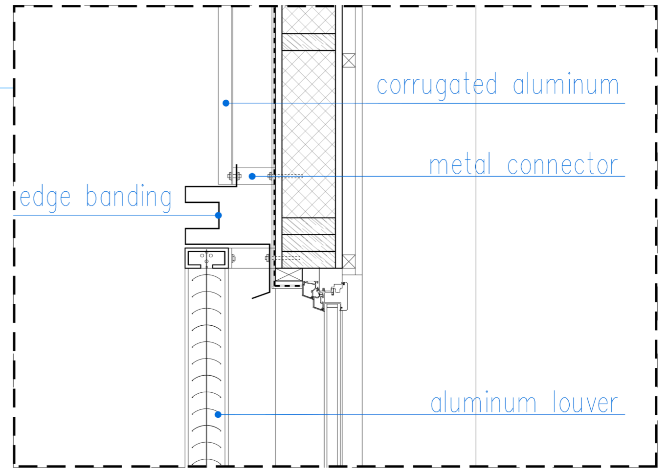
Detail of the aluminum louver
