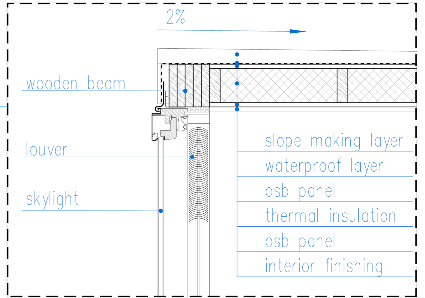
Detail of the roof layer of skylight
