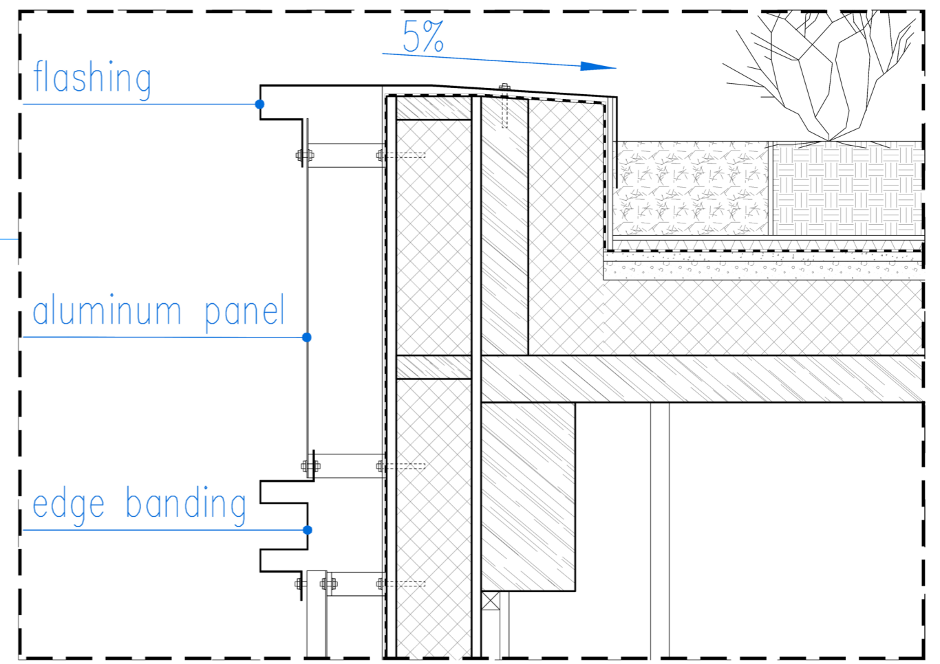
Detail of the aluminum cladding
