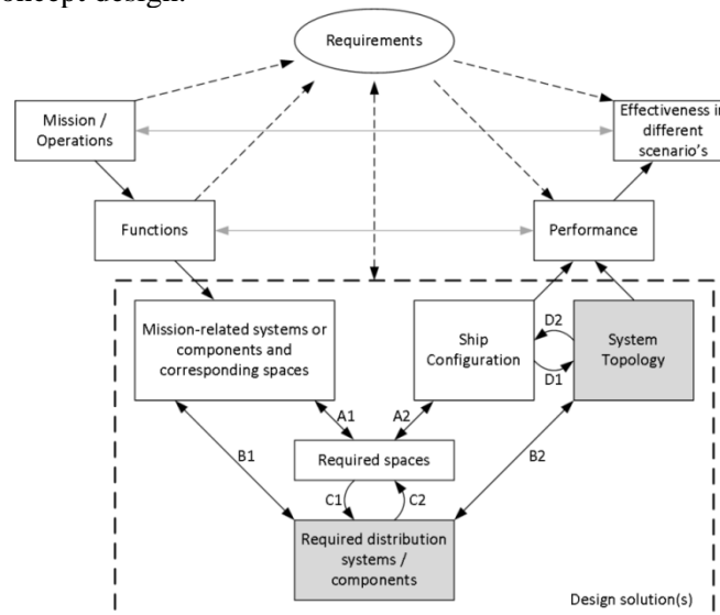
Fig.2: V-diagram representing the ship and system early stage design process
