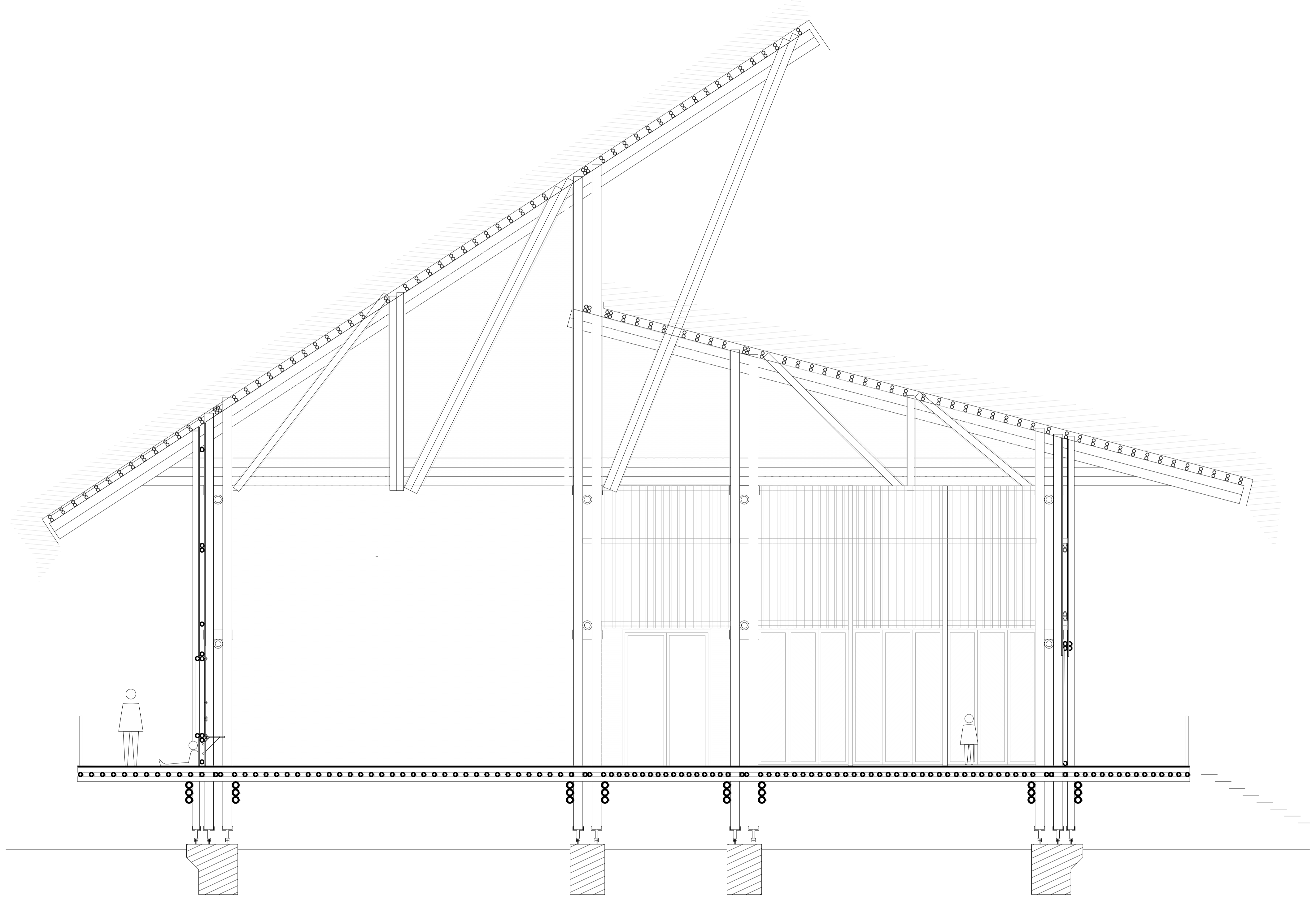
SECTION BB' - PERFORMING ARTS ROOM - 1:50
