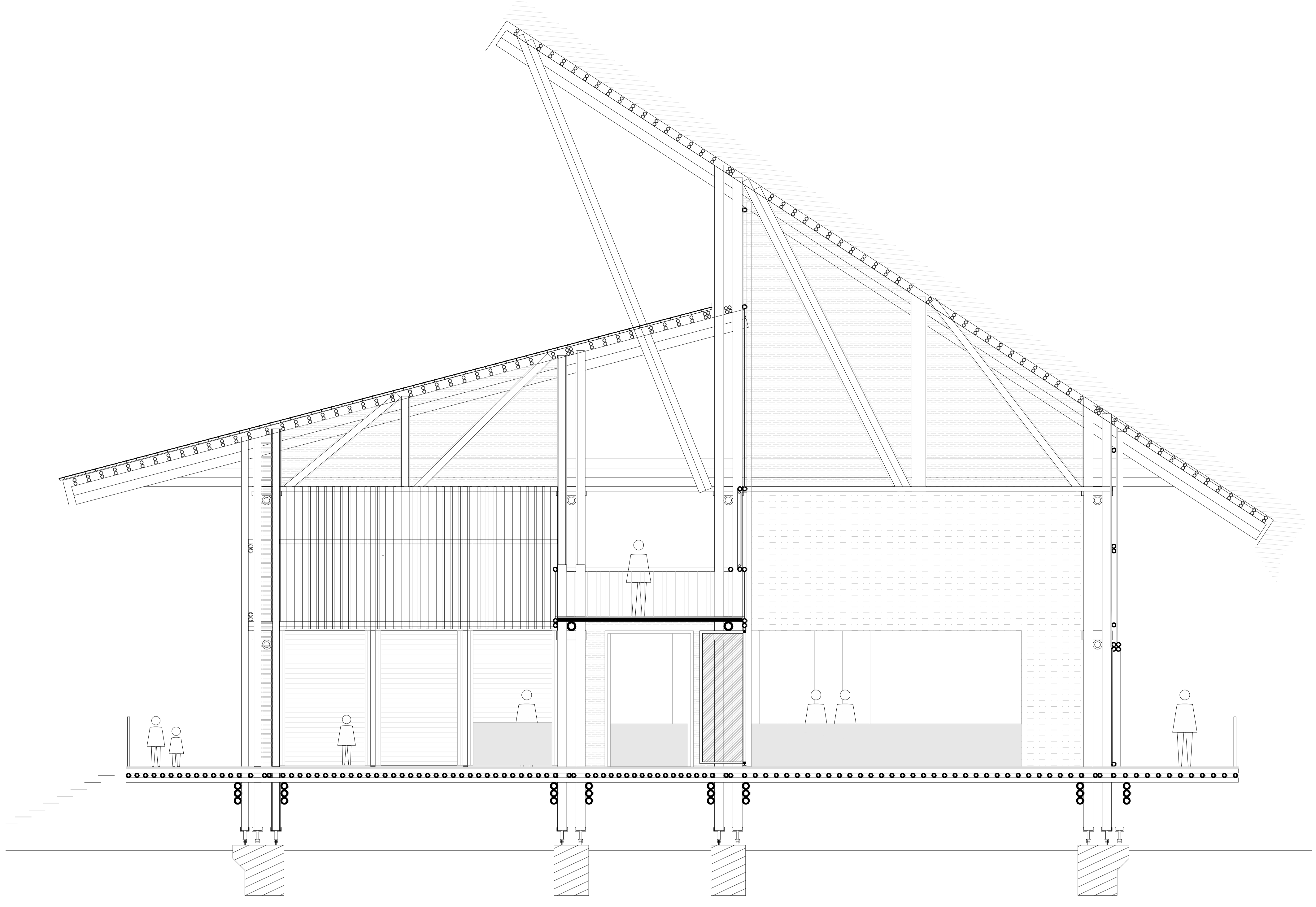
CROSS SECTION - RESTAURANT AA' - 1:50
