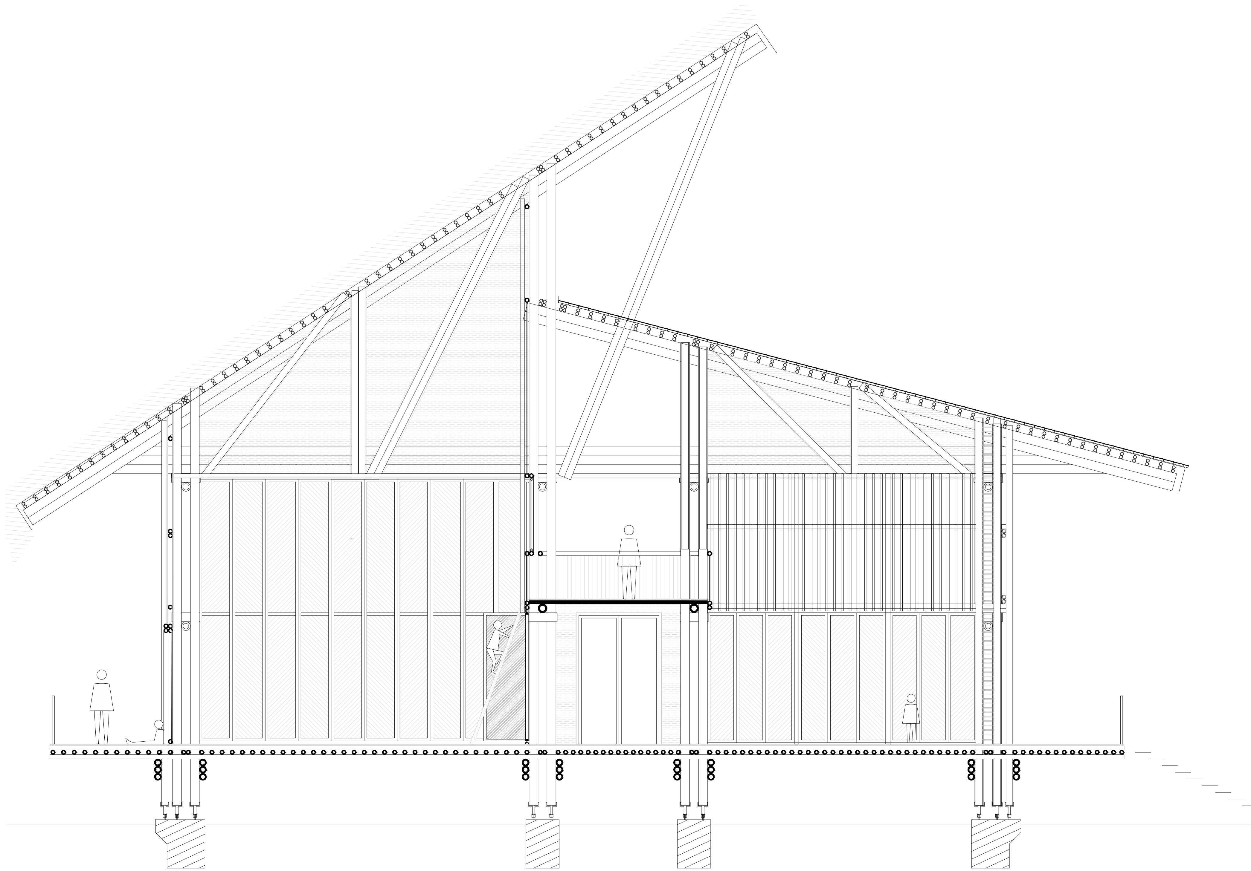
SECTION DD' - WORKSHOP & PATIO - 1:50
