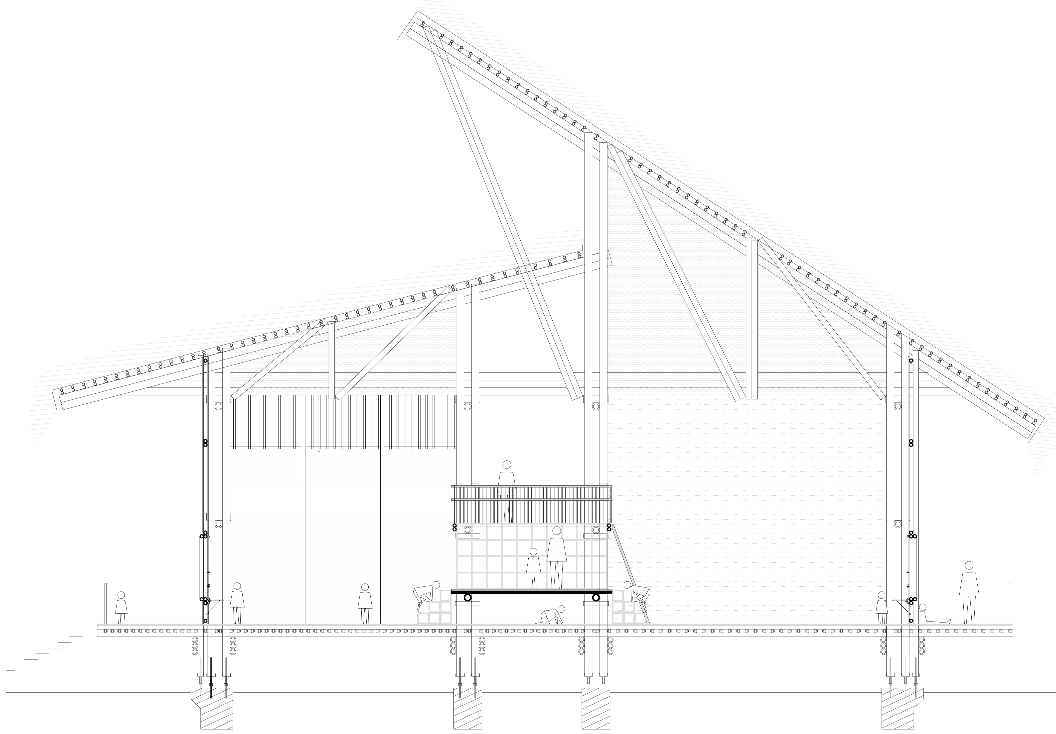
SECTION CC' - KINDERGARDEN & LIBRARY - 1:50
