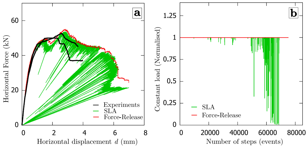
Fig. 16. Force–displacement curves of SLA and the Force-Release simulations of the smeard-crushing model, and (b) the evolution of constant load of precompression during the simulations.
