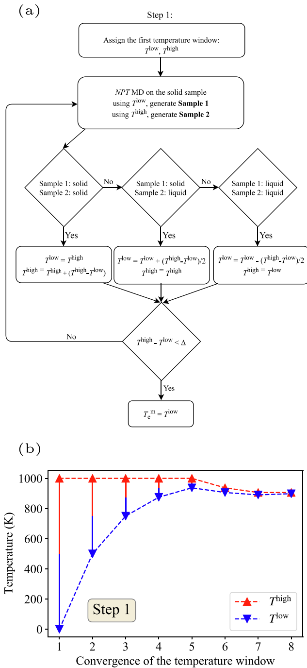
Fig. 2. (a) Schematic diagram of the automatized procedure for generating the first estimate of the melting temperature, T_c^m . (b) Convergence of the temperature windows between T^{low} and T^{high} when applying this approach. As an example, fcc Al with the TOR-TILD potential [9] has been used. The threshold temperature window between the lowest and highest temperature limit is \Delta = 10 K. The estimated melting point is \sim 898 K.
