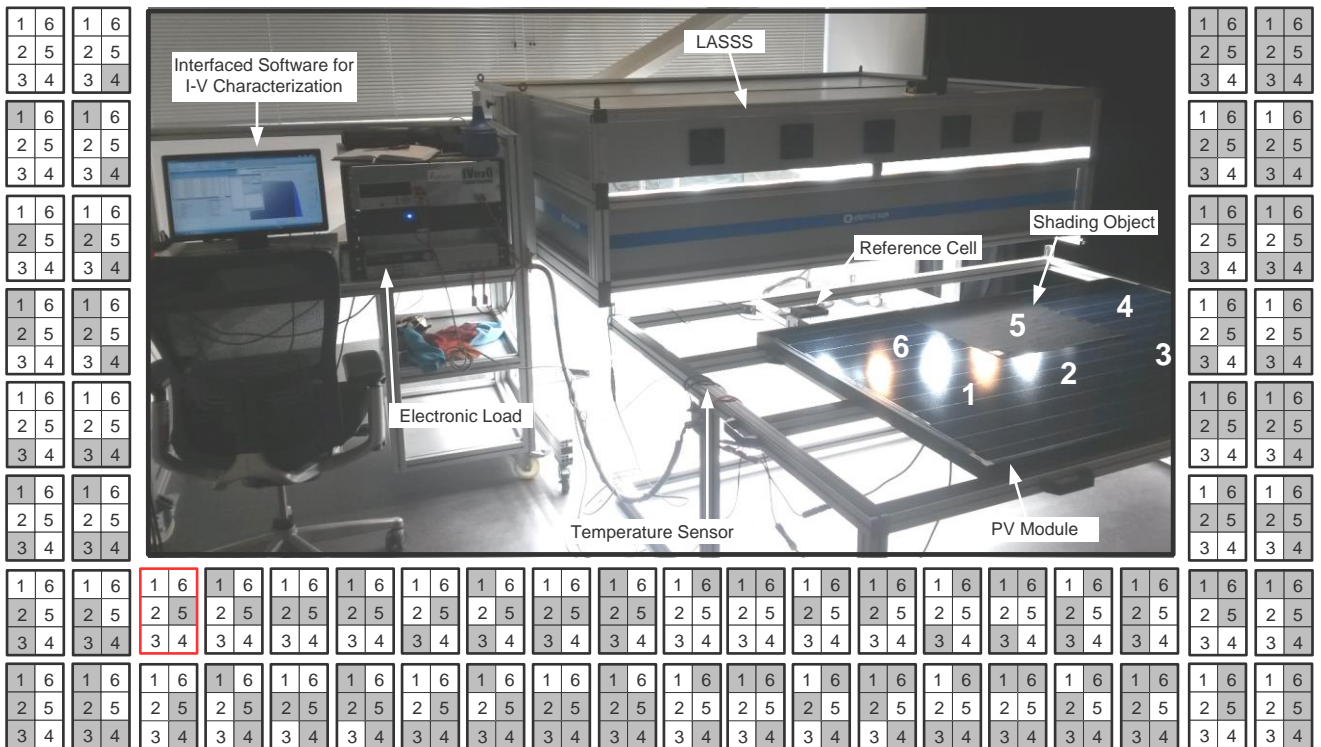
Fig. 3. Indoor experimental setup for testing shading tolerability along with 64 shading profile codes from 000000 to 111111. The depicted module under test (#4, see Table I) has 54 cells and is divided into 6 sections. The 010000 shading profile code is shown in the figure. In the figure, sections 1, 2, 3, 4, and 6 are about to receive rated irradiation ( 1000 \text{ W/m}^2 ) while section 5 is shaded and receives 250 \text{ W/m}^2 . The shading object for this specific module shades simultaneously 9 cells.
