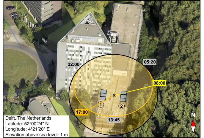
Fig. 5. Outdoor measurements location: installation location of two groups of PV modules (blue rectangles). Black x indicates the location in which outdoor experiments took place. The orange curve is the sun trajectory in June 2016, and the yellow area around (between black and orange curves) is the variation of sun trajectories during the year. According to sun path during 8.00 to 17.00, PV modules in group 2 experience shading most of the time while group 1 modules are exposed to sun. Average local times of sunset (22:00), sunrise (05:00), and solar noon (13:45) during June 2016 are also depicted to provide better perspective of the sun position during outdoor measurements.
