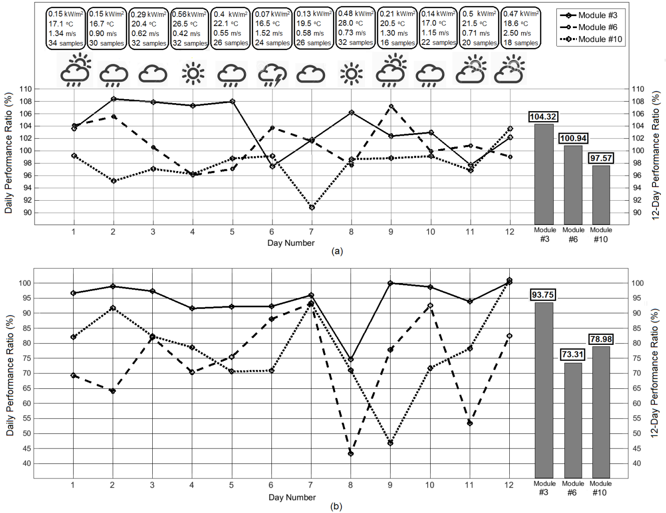
Fig. 6. Outdoor test results: (a) daily (lines) and 12-day (bars) performance ratio values for three tested PV modules exposed to sunny condition; (b) daily (lines) and 12-day (bars) performance ratio values for three tested PV modules exposed to shading condition. Weather condition are: average irradiance (at the same angle), ambient temperature, and wind speed (at modules installation altitude). Sky condition during the measurement time is also indicated. Harsh weather condition and safety policy forced us to skip sampling occasionally. Therefore, the 12-day performance ratio is calculated considering the number of samples on each day. Above hundred percent values of PR for PV modules in (a) is mostly because of the low ambient temperature. In order to obtain more accurate PR values for the modules exposed to shading condition, we did not trust in datasheet figures. Hence, for the modules in the shading-condition group, instead of datasheet nominal values, in-lab measured values of MPP at STC (1 kW/m 2 , AM 1.5, and 25 °C) is used for PR calculation (module #3 = 78.7 W, module #6 = 347.6 W, module #10 = 78.2 W). Whereas for the sunny-condition group, it was confined to datasheet values because study of modules' performance exposed to sunny condition were not the aim of the outdoor experiments.
