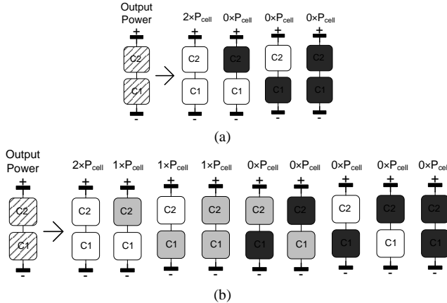
Fig. A.1. Graphical demonstration of ST formulation procedure: (a) PV module with two series-connected cells and two possible irradiation levels (0 and 1 kW/m 2 ) which results in total 2 2 working conditions, (b) PV module with two series-connected cells and three possible irradiation levels (0, 0.5, and 1 kW/m 2 ) which results in total 3 2 working conditions. Output power of PV modules at each working condition is also depicted.
