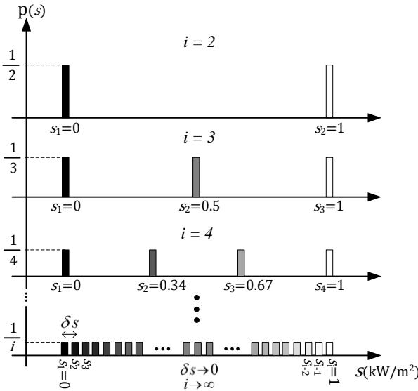
Fig. 2. Probability distributions p(s) of PV module shading problem for different number of irradiation levels i . \delta s is the difference value between two consecutive irradiation levels.
