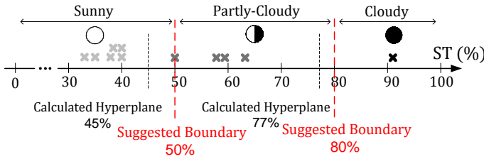
Fig. 4. Proposed shading classification boundaries for PV modules
