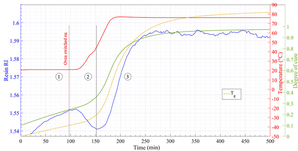
Figure 7. Comparison between \alpha and the resin RI with TC temperature and T_g evolution.
