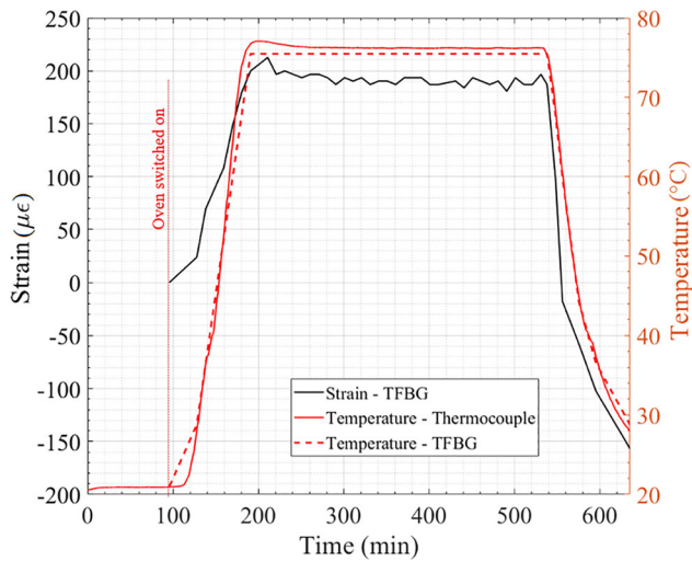
Figure 5. Temperature and strain trends during the composite curing time measured through the embedded TFBG and TC.
