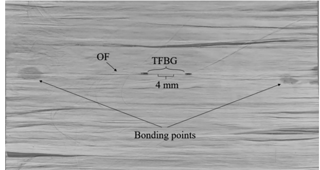
Figure 2. Positioning and gluing of a TFBG sensor on a reinforcement ply.
