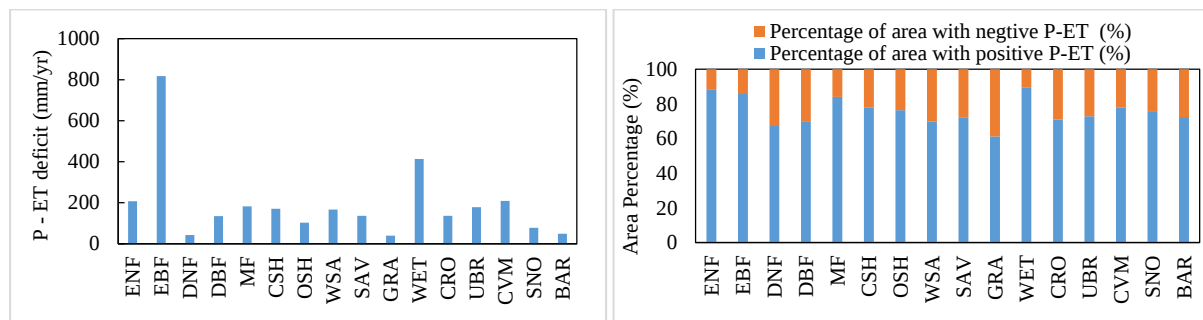
Figure 2. Variation of P-ET among different land cover types. (left panel: averaged P-ET in each land cover type; right panel: percentage of water gain and loss area for each land cover type)
