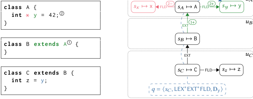
Fig. 9. Confirmation example. The left part shows a Java program, in which a field x is renamed to y . At the right side, the corresponding scope graph is shown, with the parts corresponding to the changes colored and numbered accordingly. In the program as well as in the scope graph, the color red denotes removals, while green denotes additions. In the scope graph, additions are also indicated with a plus symbol, and removals with a minus. Finally, q shows the query for y in C , which eventually resolves to A.y .
