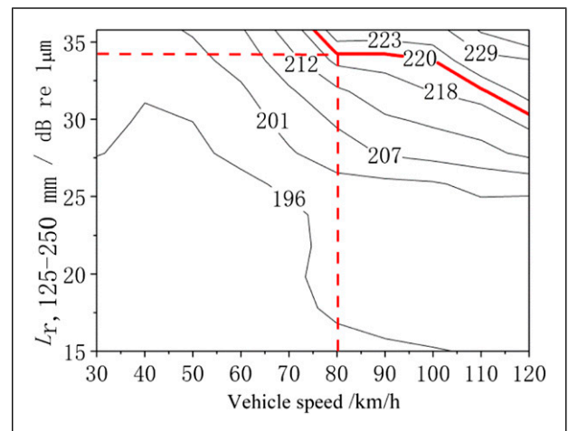
Figure 12. Influence of vehicle speed and corrugation level of 125–250 mm wavelength on wheel subsurface fatigue.
