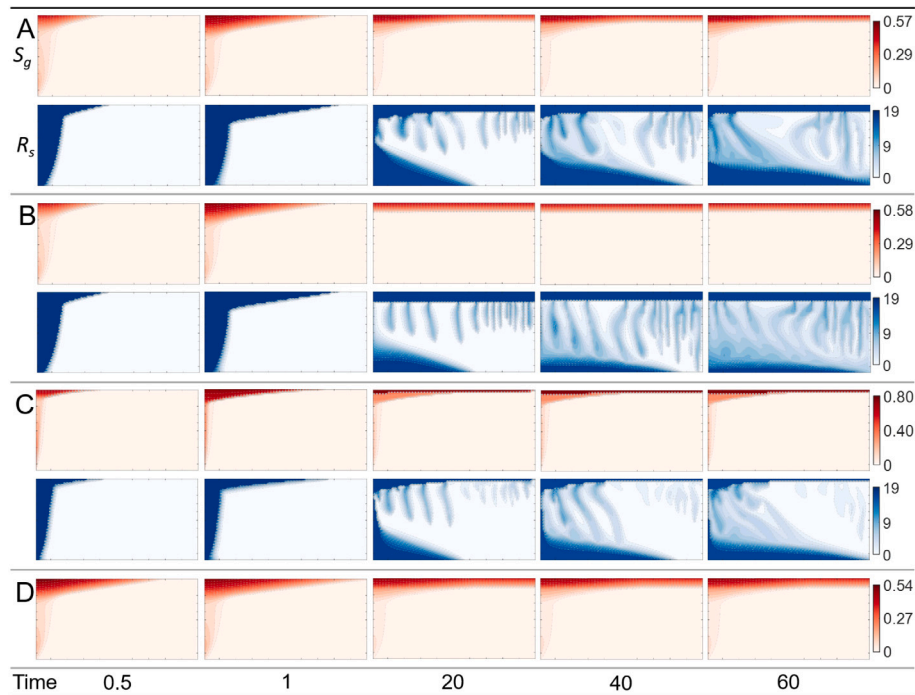
Fig. 7. Gas phase saturation and solution CO 2 -brine ratio profiles for various scenarios in a homogeneous permeability field. (A) shows results from the base case; (B), (C), and (D) present results from the case without hysteresis, capillary pressure, and dissolution, respectively. (D) includes saturation maps only because the solution ratio is zero at all times.
