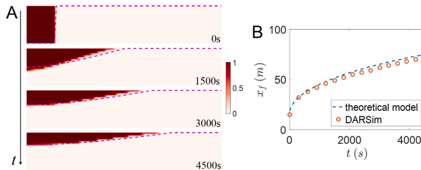
Fig. 5. (A) Saturation maps of the buoyant fluid obtained from numerical simulations, along with predictions of the theoretical model (dashed lines) at t = 0s, 1500s, 3000s, and 4500s. (B) Leading position of the buoyant current obtained from numerical simulations (circles) and the theoretical model (dashed line).
