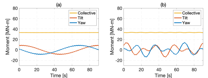
Fig. 3. Moment signals in the fixed frame for simulation cases of (a) SS (b) MS. The collective, tilt, and yaw moments are represented by the yellow, orange and blue line, respectively.
