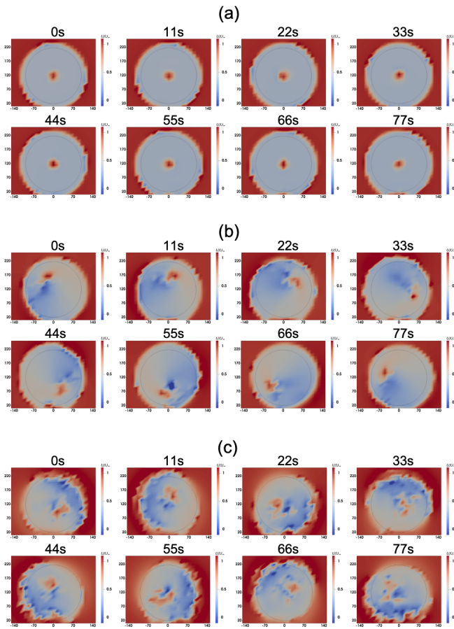
Fig. 6. The normalized velocity field behind the rotor at the distance of 1D seen from the front view at different time instances for simulation cases of (a) BL (b) SS and (c) MS. The horizontal and vertical dimensions are expressed in the unit of meters. The red area represents higher wind velocity and the black circle represents the rotor region projected on the 1D plane.
