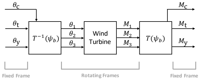
Fig. 1. The framework of the Helix approach. The individual pitch actuation signals in the rotating frames, \theta_1 , \theta_2 and \theta_3 , are implemented on each blade, and these pitch perturbations are assumed to result in the amplitude-scaled and phase-shifted responses of moment signals on blade roots with the same frequency content, expressed by M_1 , M_2 and M_3 . The multi-blade coordinate (MBC) transformation, T , as a function of the azimuth position of each blade, \psi_b , is implemented on the moment signals to obtain the combined effects of these rotating-frame moment signals on the fixed frame, which are expressed in the tilt and yaw directions, M_t and M_y . The fixed-frame collective moment M_c is also obtained. In a similar manner, the rotating-frame pitch actuation signals can be obtained through the implementation of the inverse MBC transformation, T^{-1} , on the collective, tilt and yaw pitch actuation signals on the fixed frame, \theta_c , \theta_t and \theta_y . The relationship between the pitch actuation signals and the moment signals on the fixed frame is obtained through the overall framework. It is noted that a nonzero presence of M_t and M_y implies that the thrust force is not acting on the rotor center. In other words, the position of the thrust force on the rotor can be dynamically manipulated by implementing the time-varying pitch actuation signals, which is considered an effective way to dynamically deflect the wake.
