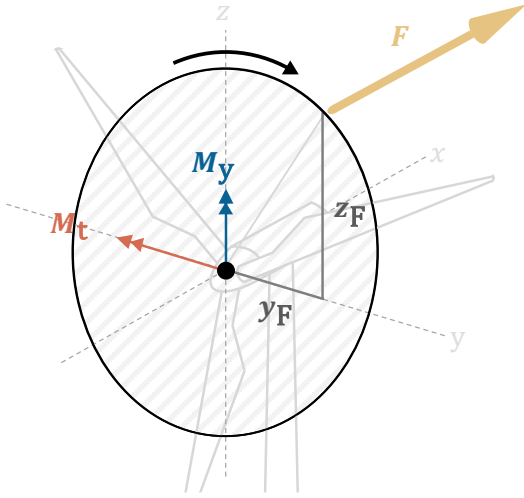
Fig. 2. The illustration of the thrust force manipulation in the Helix approach. The fixed-frame pitch actuation signals \theta_t and \theta_y are implemented and induce the corresponding fixed-frame moments M_t and M_y on the rotor. The distance between the thrust force F and the rotor center is defined by italic y_F and z_F . The black line represents the trajectory of the thrust force. By implementing specific combinations of \theta_t and \theta_y , the position of the thrust force is dynamically manipulated, which aims to result in wake deflection and thereby enhancing wake mixing. It is noted that the shown trajectory of the thrust force position is enlarged for the purpose of illustration.
